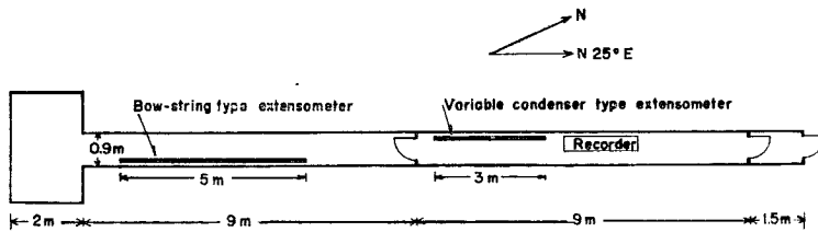
Fig. 5. Horizontal tunnel of the Kamigamo Geodesic Observatory.
