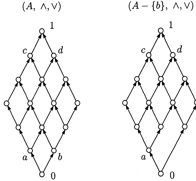
a and b are atoms, c and d are dual atoms. Hence, a, b, c and d are one-point-deletable points in (A, \wedge, \vee) .
