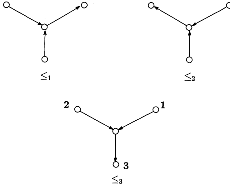
Figure 5: Example of non t-c trice
