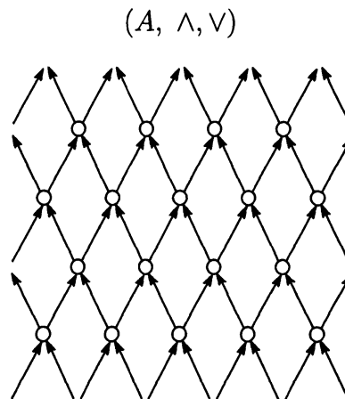
Figure 2: Example of no one-point-deletable point (infinite lattice)
