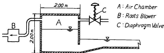
Fig. 1. Experimental facilities.
