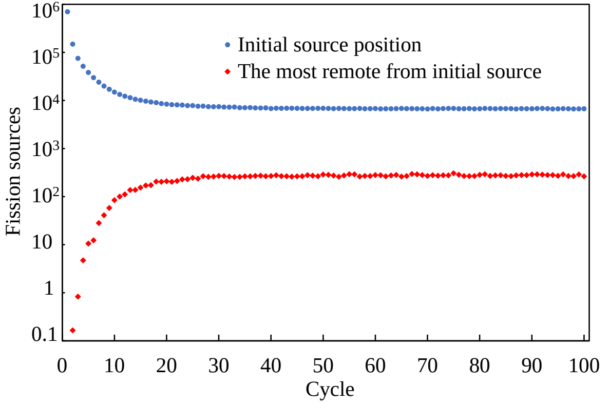
Fig. 2 Fission source convergence in Case 1
