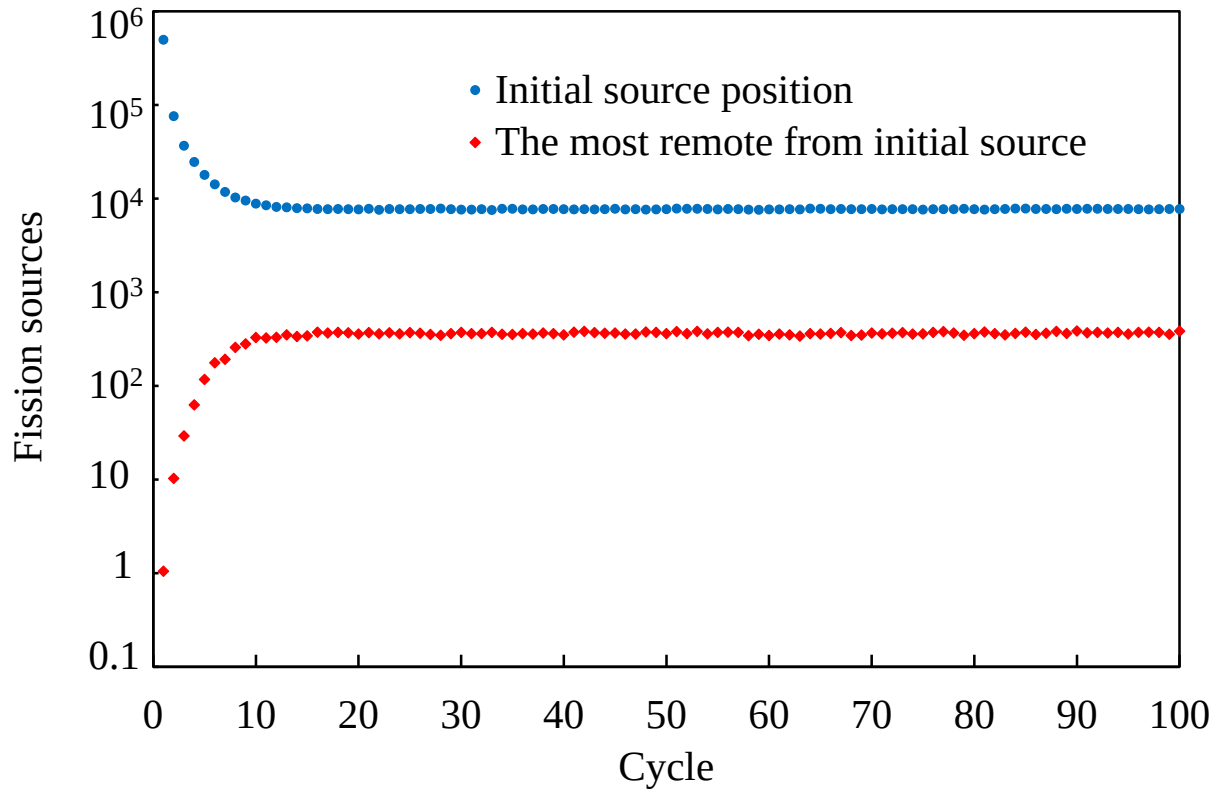
Fig. 7 Fission source convergence in Case 2
