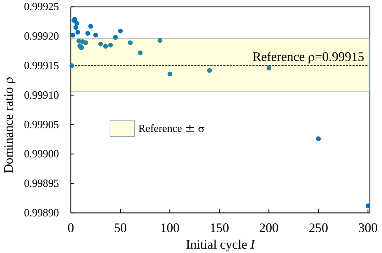
Fig. 13 Dominance ratio vs. initial cycle I in Case 3 ( r = 30 )
