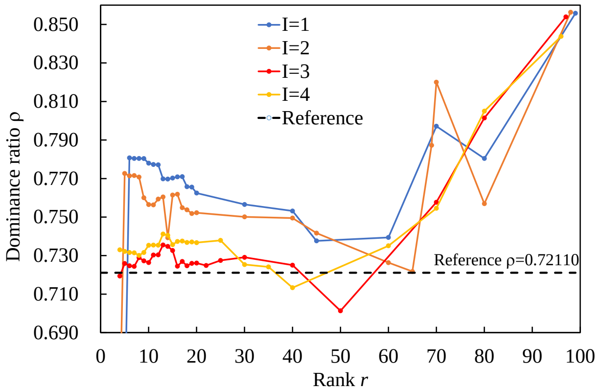
Fig. 8 Dominance ratio vs. rank r in Case 2
