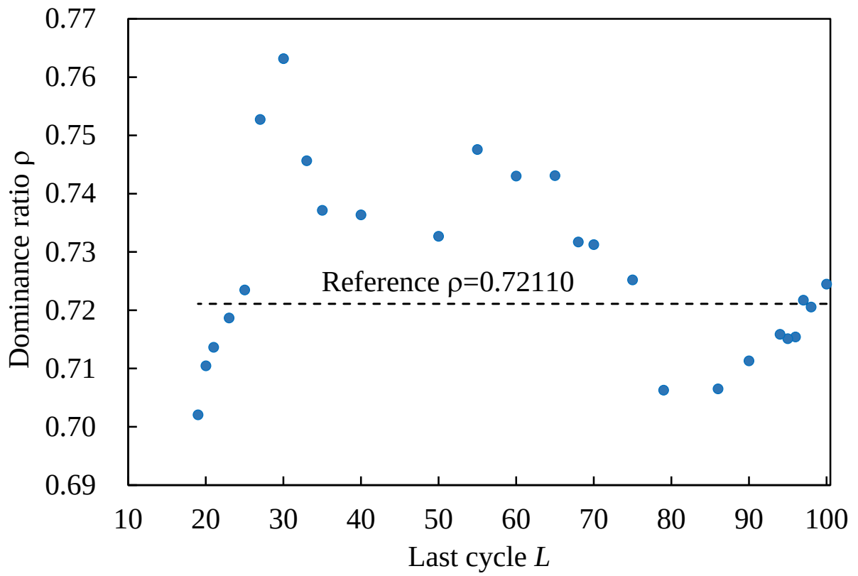
Fig. 10 Dominance ratio vs. last cycle L in Case 2 ( r = 16 )
