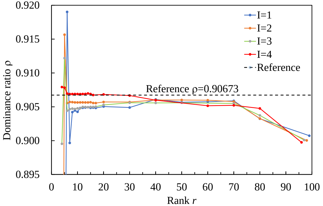
Fig. 3 Dominance ratio vs. rank r in Case 1
