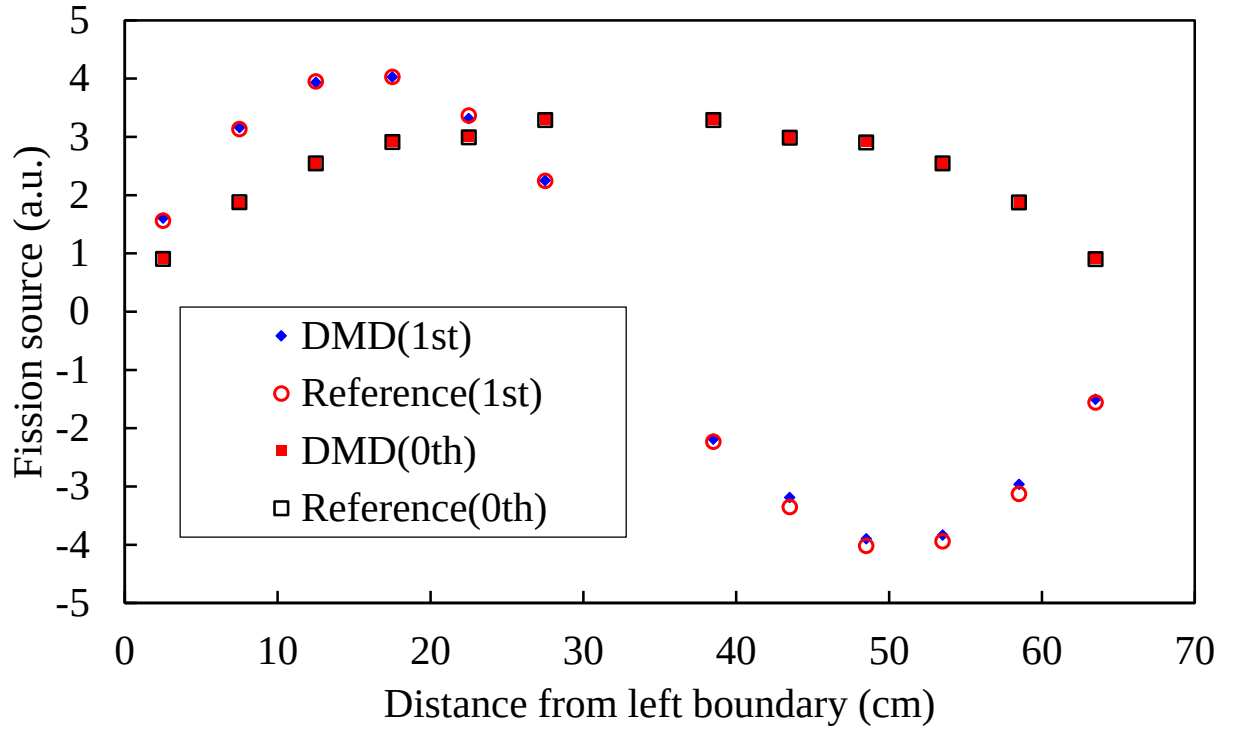
Fig.6 Normalized fission source distributions of fundamental and 1st eigenmode by DMD and eigenvalue calculation in the innermost tally region
