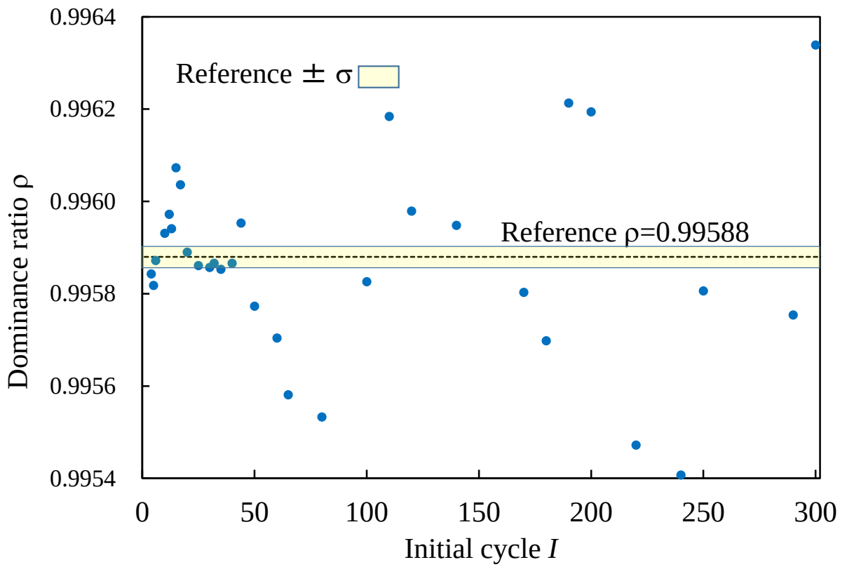
Fig. 19 Dominance ratio vs. initial cycle I in Case 4 ( r = 30 )
