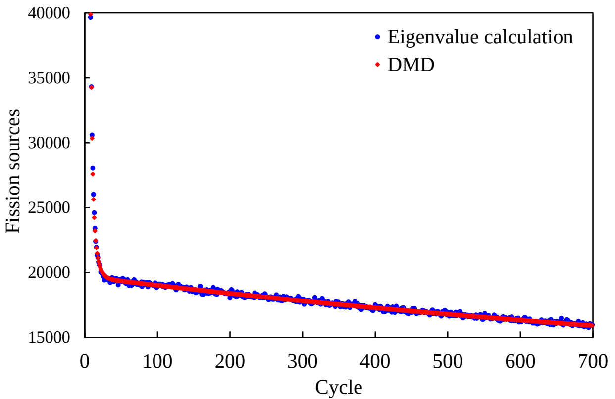
Fig. 15 Fission source transition that was reconstructed by the DMD method in Case 3 at the fission source position
