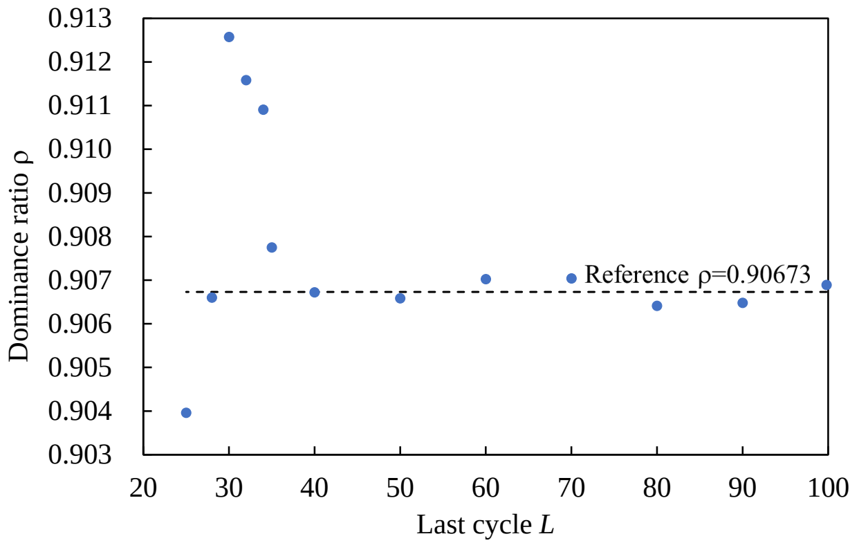
Fig. 5 Dominance ratio vs. last cycle L in Case 1 ( r = 15 )
