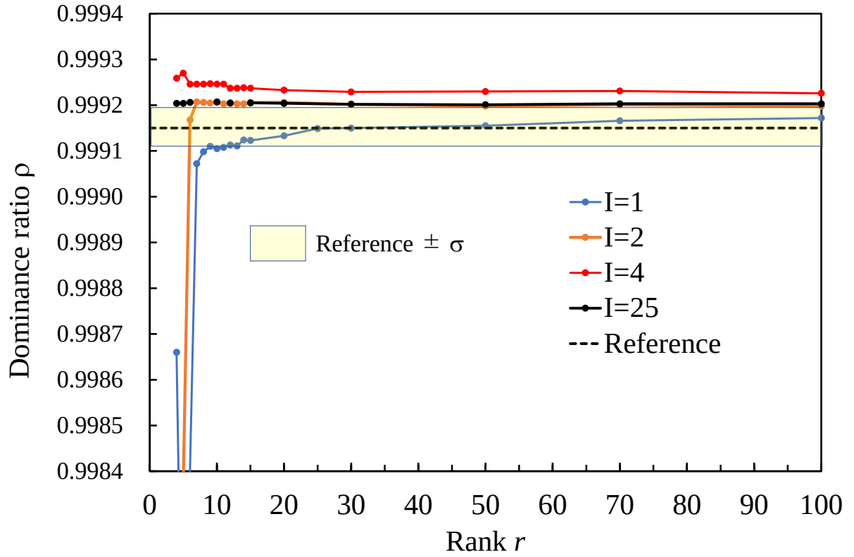
Fig. 12 Dominance ratio vs. rank r in Case 3
