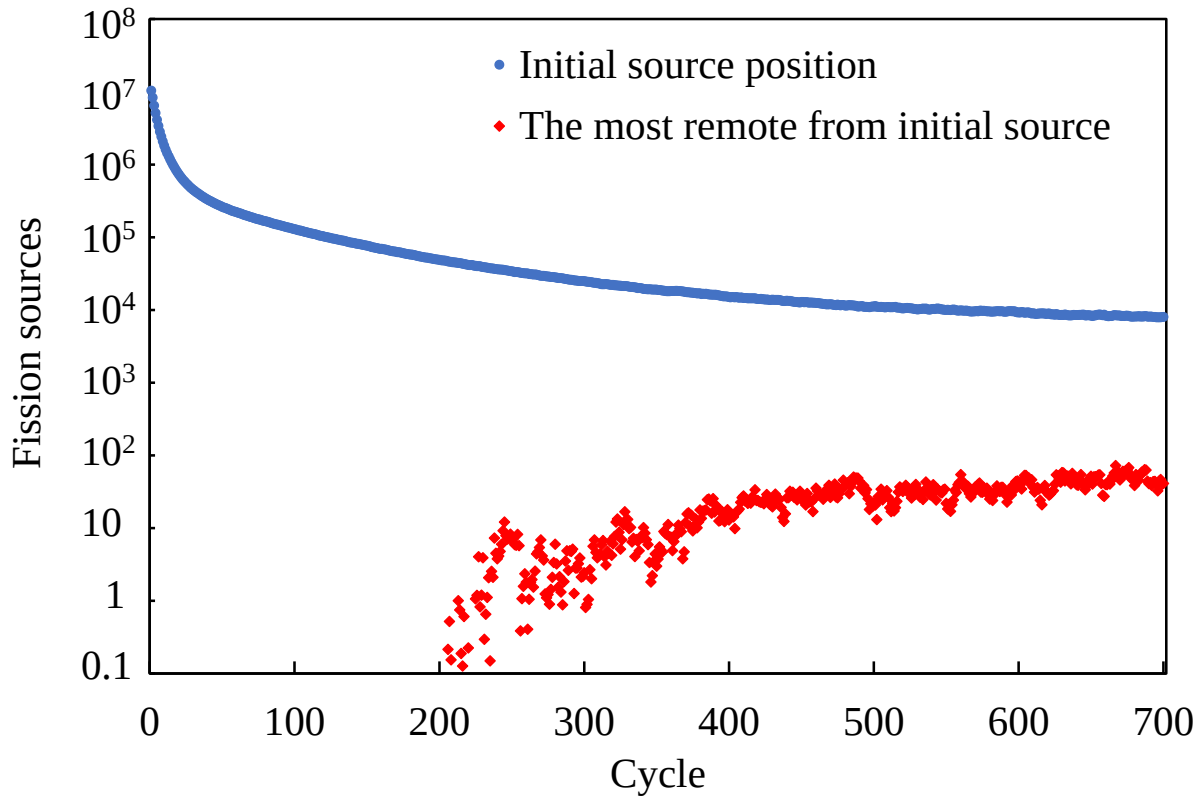
Fig. 17 Fission source convergence in Case 4
