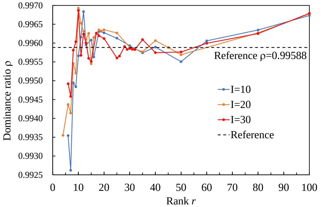
Fig. 18 Dominance ratio vs. rank r in Case 4
