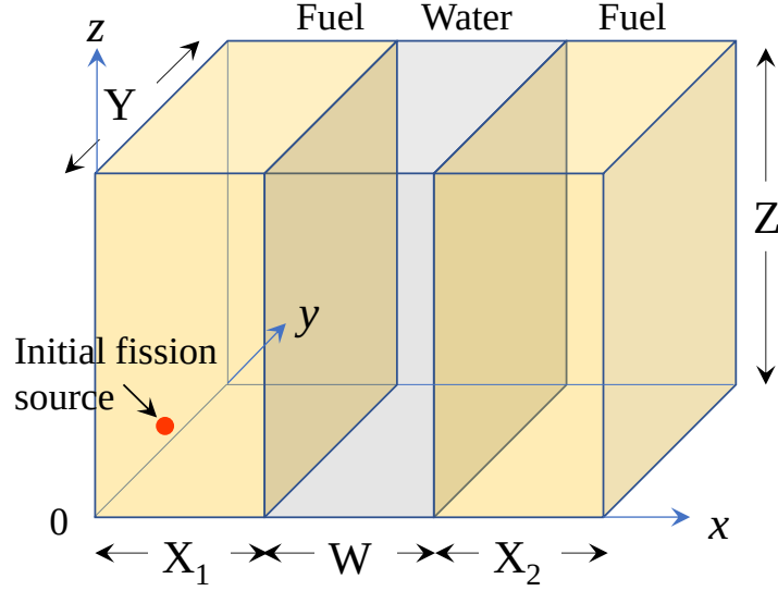
Fig. 1 Geometry for the numerical tests for Cases 1 and 3
