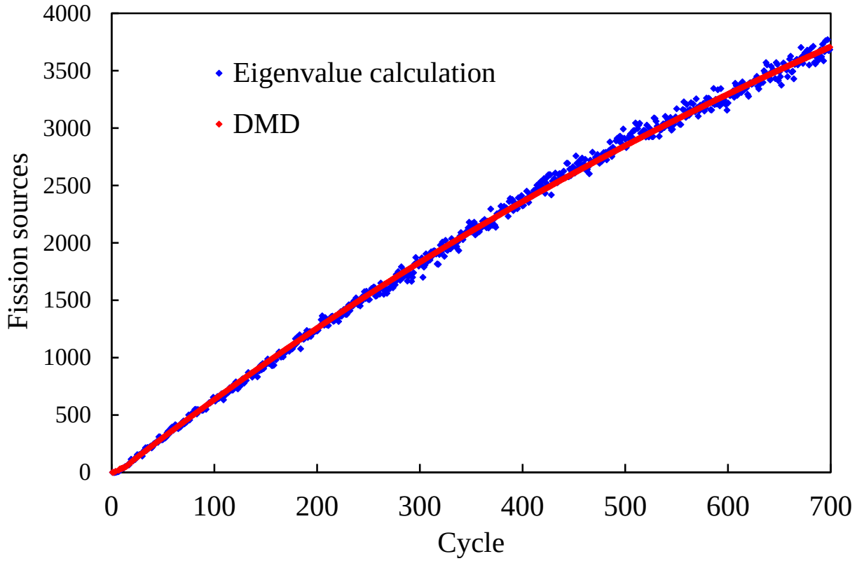
Fig. 16 Fission source transition that was reconstructed by the DMD method in Case 3 at the most remote position from the initial fission source
