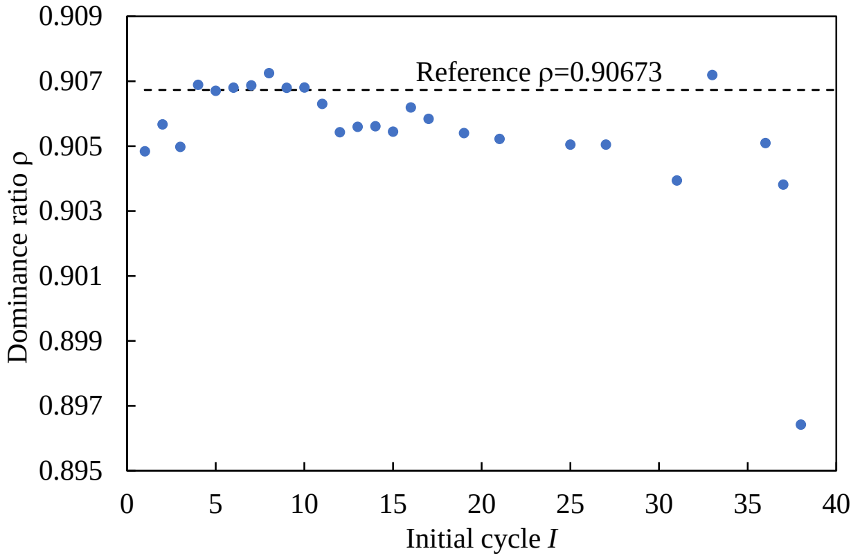
Fig. 4 Dominance ratio vs. initial cycle I in Case 1 ( r = 15 )
