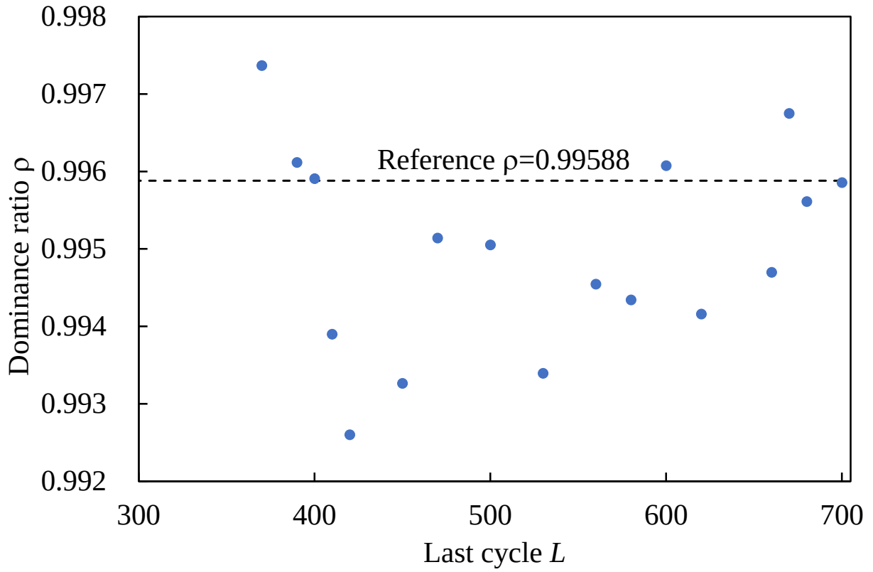
Fig. 20 Dominance ratio vs. last cycle L in Case 4 ( r = 30 )
