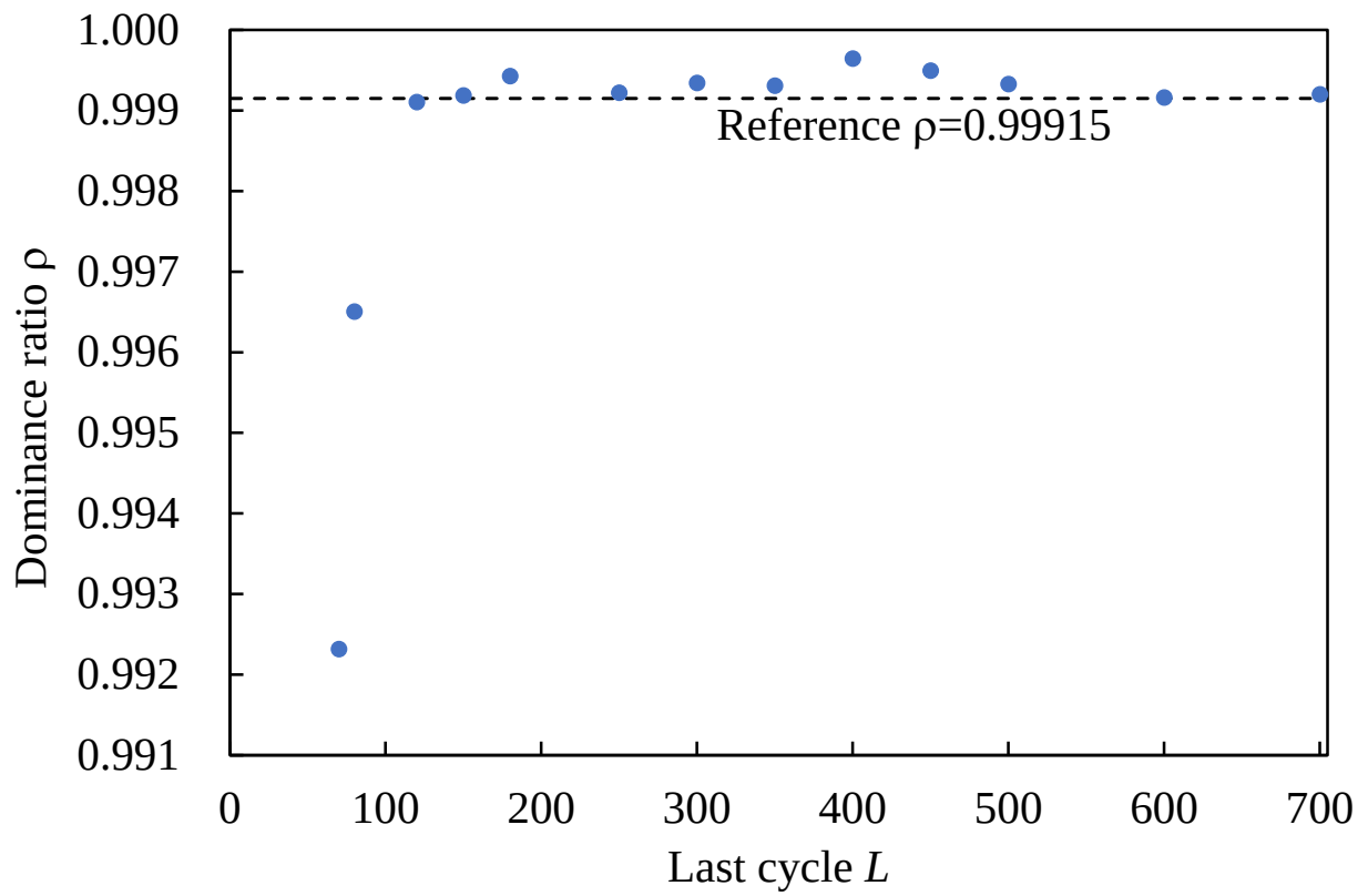
Fig. 14 Dominance ratio vs. last cycle L in Case 3 ( r = 30 )
