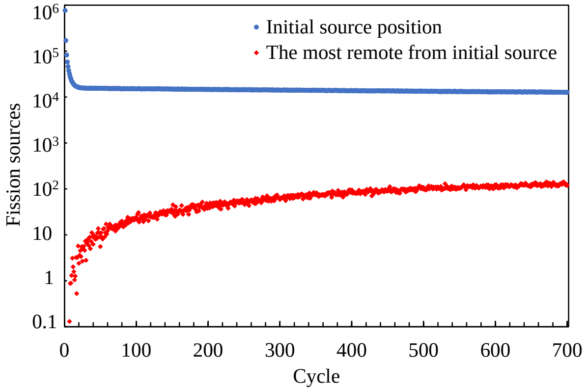
Fig. 11 Fission source convergence in Case 3
