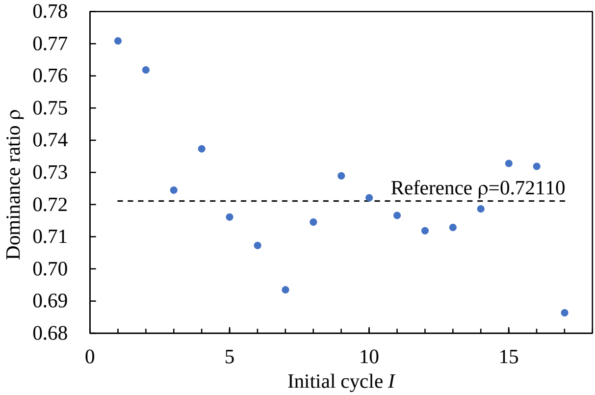
Fig. 9 Dominance ratio vs. initial cycle I in Case 2 ( r = 16 )
