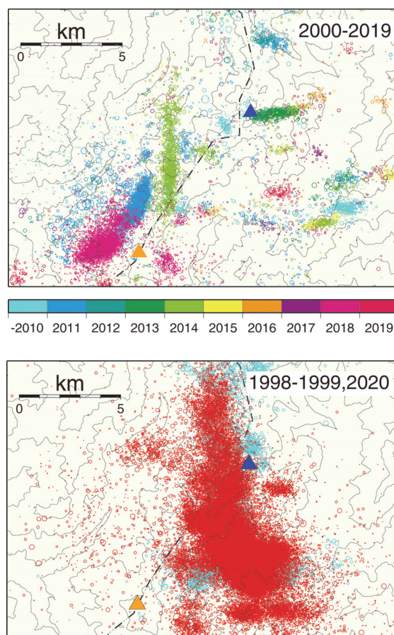
Fig.10: (a) (upper) Yearly plot of the seismicity since 2000 until 2019. (b) (lower) Seismicity of 2020 activity (red dots) together with that of 1998 (1998-1999) (cyan dots). Dashed line shows the main ridge line of Hida mountain range, which is also the prefecture border of Gifu and Nagano prefectures. Blue and orange triangles shows Mts. Okuhotaka-dake and Yake-dake, respectively.
