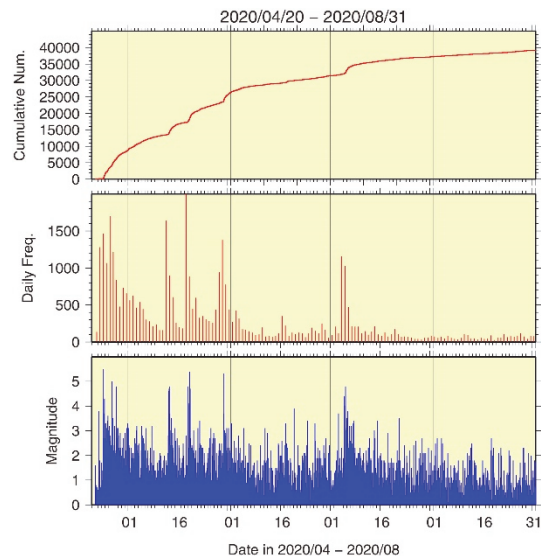
Fig.3: Seismic activity of the swarm in 2020. Cumulative number (upper), daily frequency (middle), and magnitude time diagram (lower) of the earthquakes located in the area of Fig.2 (a) are shown. All earthquakes documented in the JMA catalogue are used.
