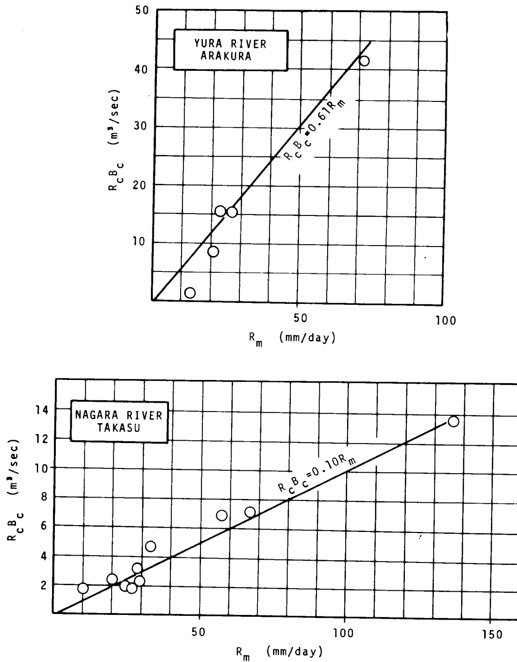
Fig. I-19 Relationship between Value R_c B_c and Mean Daily Rainfall R_m (Confined Component)
