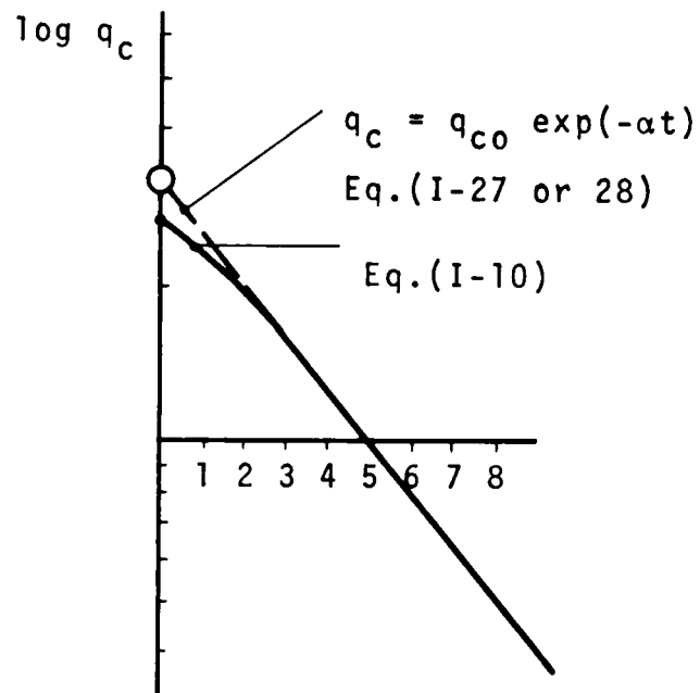
Fig. I-4 Graphical Explanation of Eq. (I-10) and Eq. (I-27)
