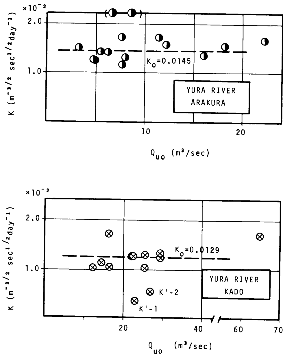
Fig. I-13 Recession Factor K versus Initial Discharge of Unconfined Component
