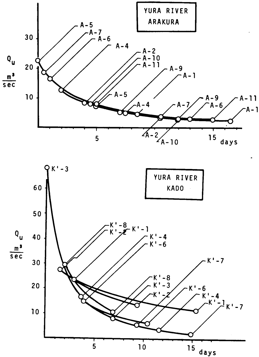
Fig. I-15 Recession Curve of Unconfined Component in (t, Q_u) -plane
