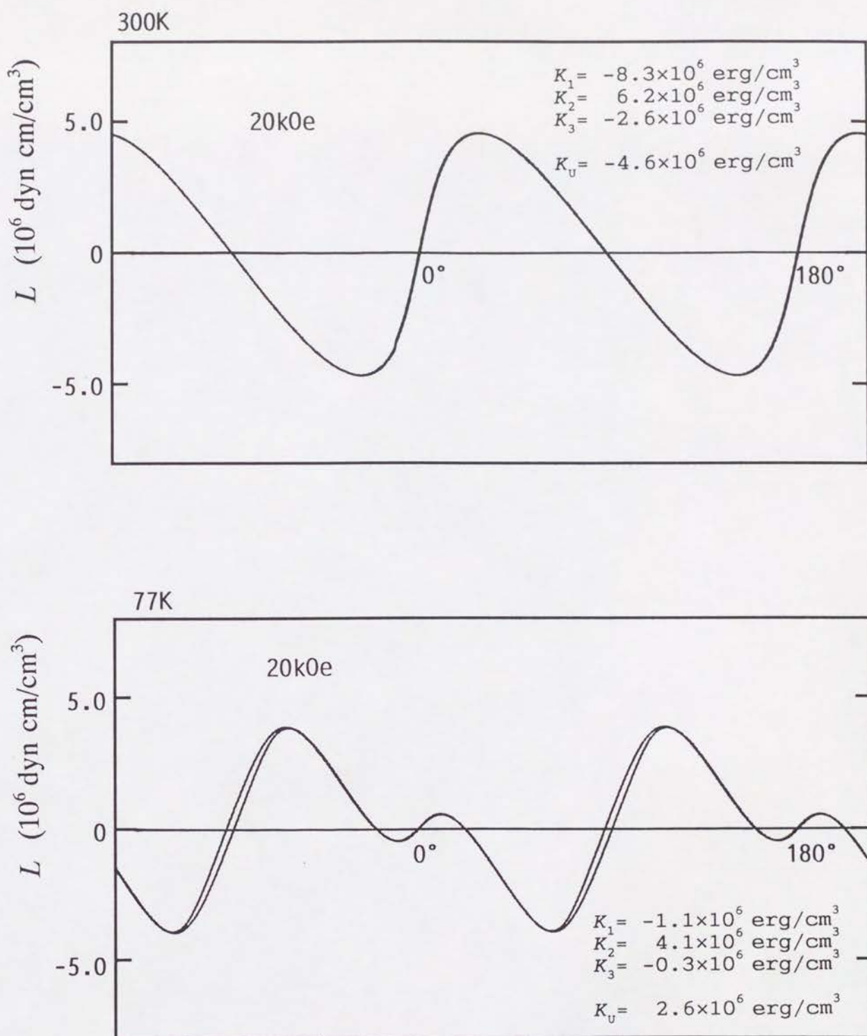
Fig. 69. Torque curves for [Fe(26Å)/Nd(28Å)] at 300K and 77K. For a rough estimation of the anisotropy constants K_1 , K_2 , K_3 , and K_v , the curves were fitted with a single magnetic component with uniaxial anisotropy energy expressed by eq. (6).
