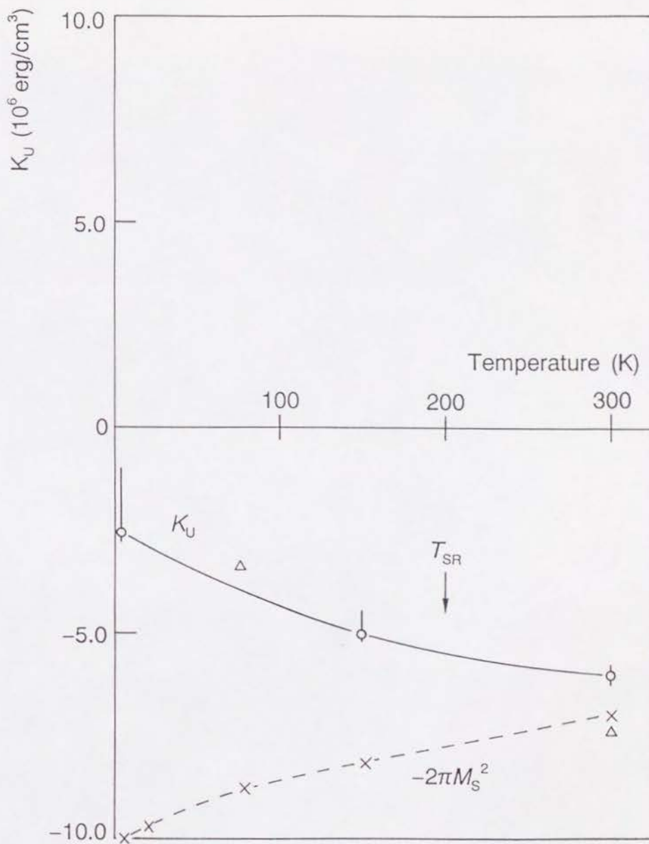
Fig. 65. Temperature dependence of the magnetic anisotropy constant K_u estimated from magnetization measurements (O) and torque measurements ( \Delta ) for [Fe(39Å)/Nd(28Å)]. The shape anisotropy energy -2\pi M_s^2 is also shown for comparison (x). The temperature where the spin reorientation is observed in Mössbauer spectra is expressed as T_{SR} .
