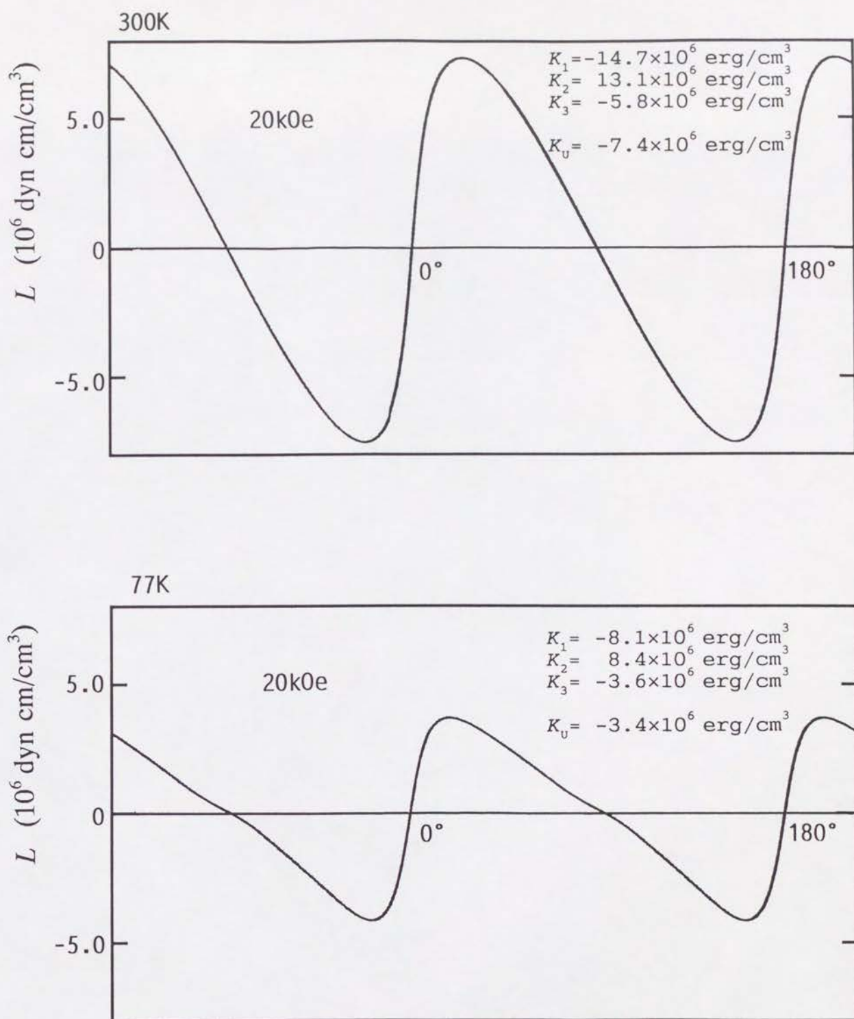
Fig. 66. Torque curves for [Fe(39Å)/Nd(28Å)] at 300K and 77K. For a rough estimation of the anisotropy constants K_1 , K_2 , K_3 , and K_v , the curves were fitted with a single magnetic component with uniaxial anisotropy energy expressed by eq. (6).
