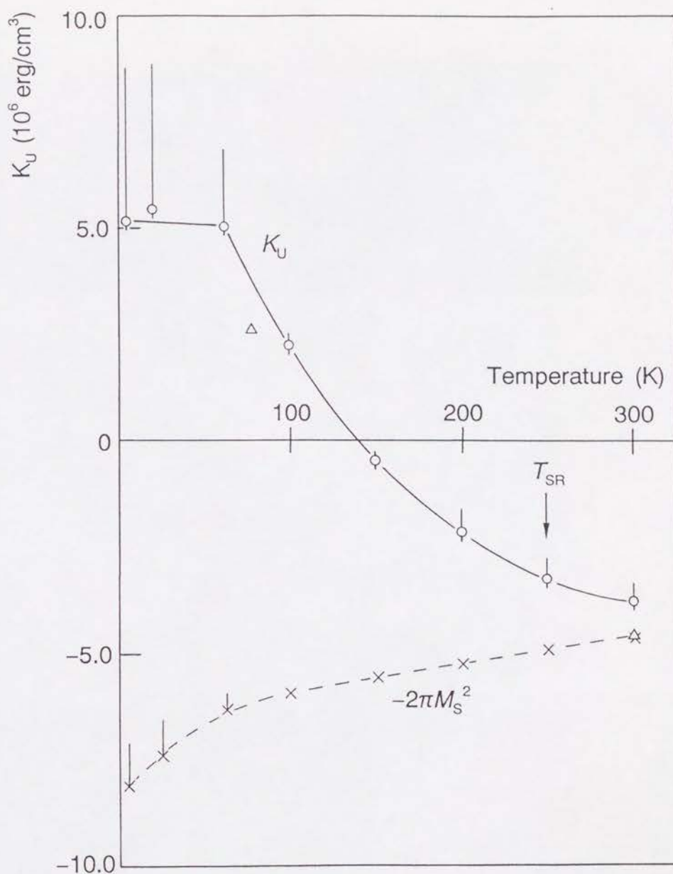
Fig. 68. Temperature dependence of the magnetic anisotropy constant K_u estimated from magnetization measurements ( \circ ) and torque measurements ( \Delta ) for [\text{Fe}(26\text{\AA})/\text{Nd}(28\text{\AA})] . The shape anisotropy energy -2\pi M_s^2 is also shown for comparison ( \times ). The temperature where the spin reorientation is observed in Mössbauer spectra is expressed as T_{SR} .
