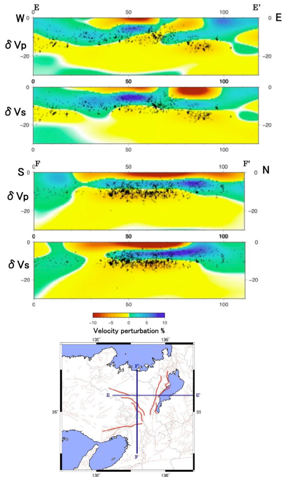
Fig. 7 Vertical cross sections of results of tomography with 0.1 degree resolution. Vp perturbation along EW line, Vs perturbation along EW line, Vp perturbation along NS line, Vs perturbation along NS line, and location of section lines, up to bottom respectively.
