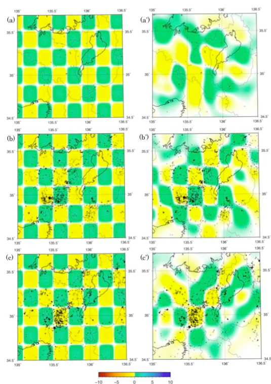
Fig. 5 Results of the checkerboard resolution tests of 0.1 \times 0.1 degree grid interval for P wave on three representative depth layers; (a) 1km, (b) 7km, (c) 13km Left side panels are true checker model, right side panels are recovered model respectively.
