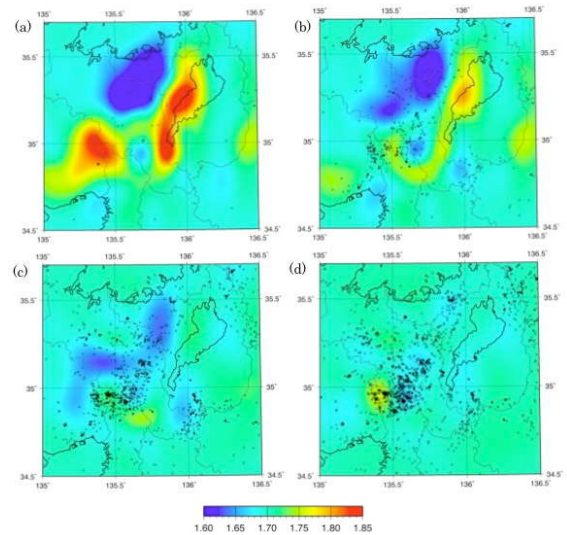
Fig. 8 Vp/Vs distributions on the results of tomography with 0.1 degree resolution. Map view at the depth of (a)1km, (b)4km, (c)7km and (d) 10km, respectively.
