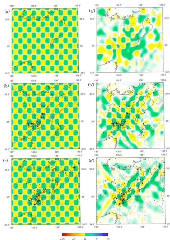
Fig. 6 Results of the checkerboard resolution tests of 0.05 \times 0.05 degree grid interval for S wave on three representative depth layers; (a) 1km, (b) 7km, (c) 13km Left side panels are true checker model, right side panels are recovered model respectively.
