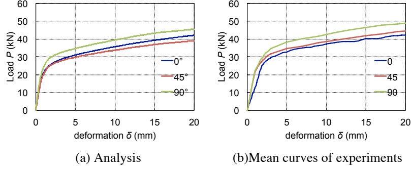
Fig.8 Example of P - \delta curves that obtained by analysis and experiment.
