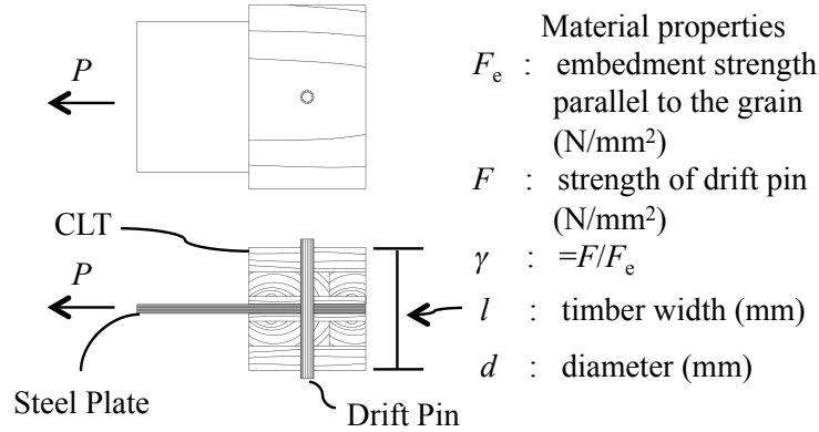
Fig. 1 Concept of joint and defenition of material properties.
