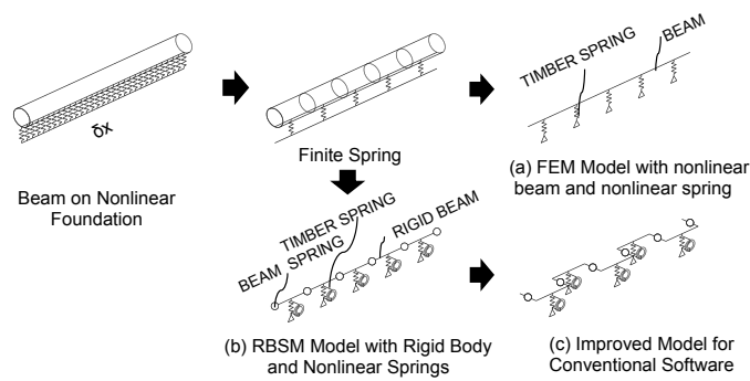
Fig.5 Comparing between FEM model and RBSM model.
