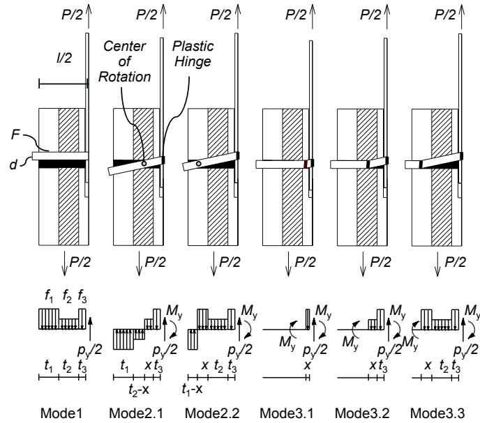
Fig.2 Possible yielding models based on equilibrium of the loads.
