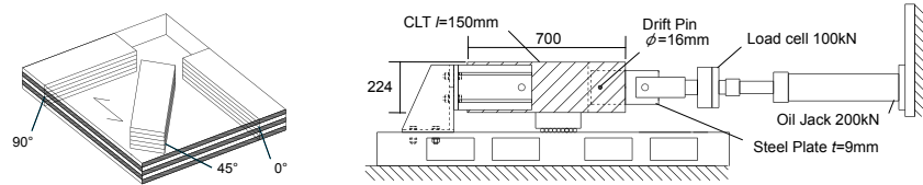
Fig.6 Sampling of specimens and apparatus of tensile test for CLT - drift pin joint.
