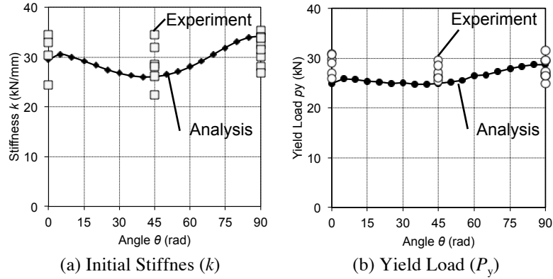
Fig.9 Comparison in characteristics between analysis and experiment.
