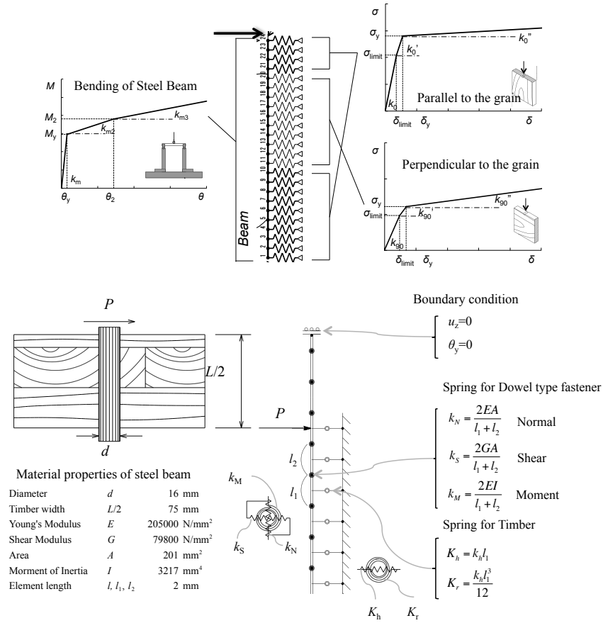
Fig.4 Numerical Analysis Model (RBSM) for the half of the drift pin joint.
