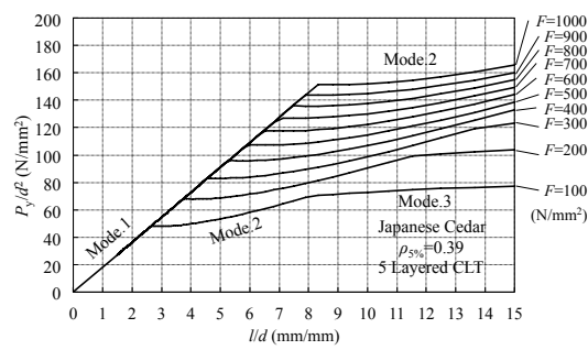
Fig. 3 Relationships ( P_y/d^2 - l/d ) for the Load Carrying Capacity ( p_y ).
