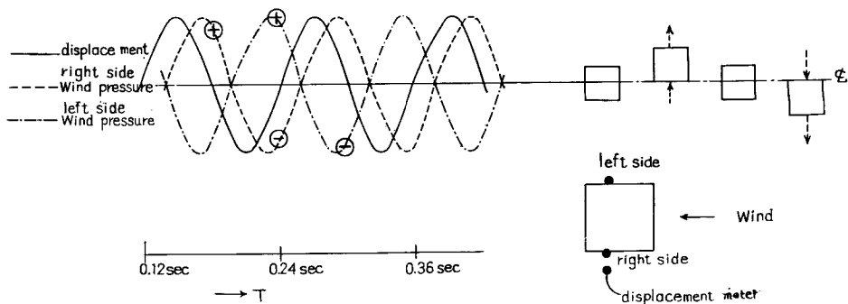
Fig. 4 Relation between phase lag of wind pressure and displacement of a moving cylinder.
