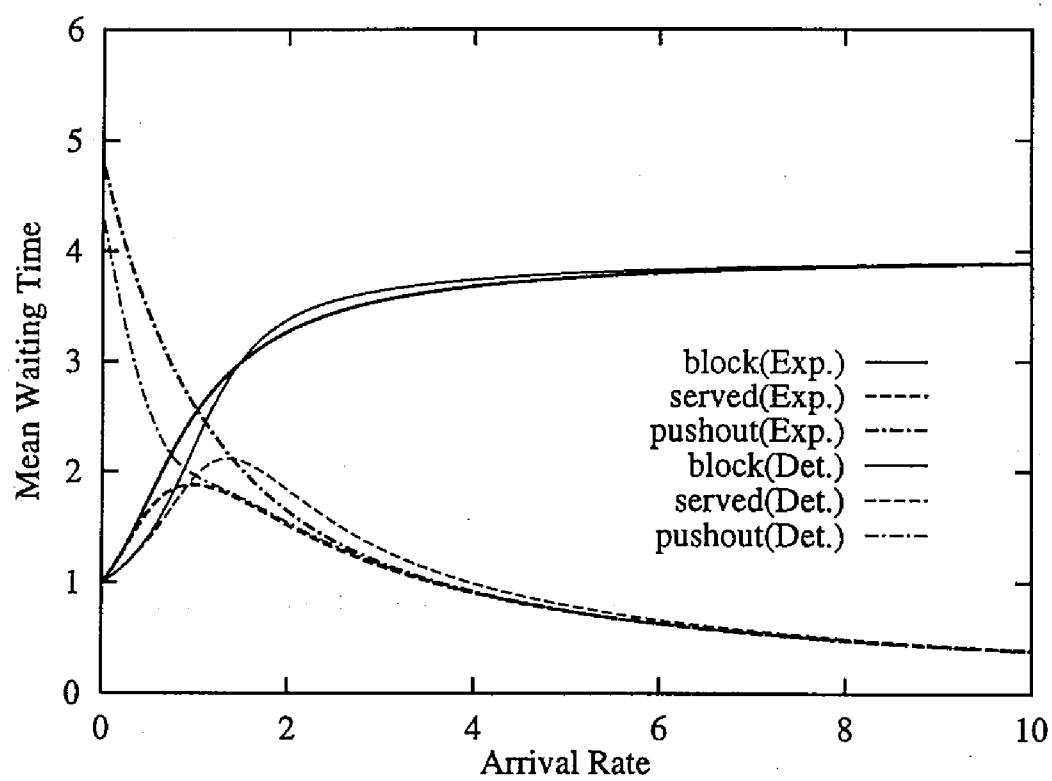
Figure 4.3: Mean Waiting Time under FCFS
