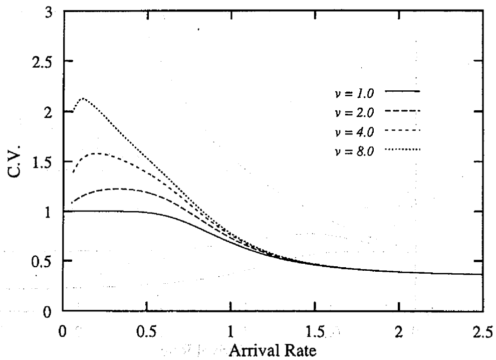
Figure 3.4: C.V. under FCFS ( K = 10 , k = 1 ) : \rho = 0.5 , \sigma = 0.5
