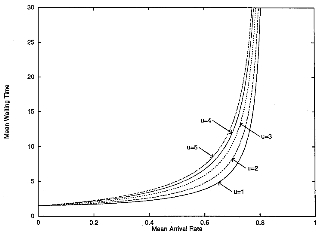
Figure 5.2: Mean Waiting Time of an SPP/G/1 System
