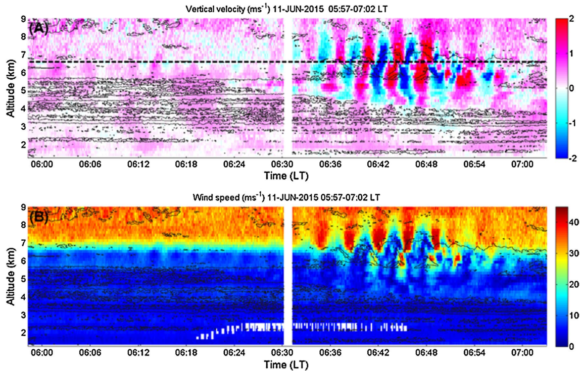
Fig. 4 a Time–height cross section of vertical velocity W ( \text{ms}^{-1} ) measured by the vertically pointing beam of the MU radar. The horizontal dashed line shows the altitude of the critical level of the KH instability (defined as the altitude where phase shift of W disturbances was observed). b The corresponding time–height cross section of horizontal wind speed ( \text{ms}^{-1} ). The black contours show an arbitrary level of radar echo power for delineating the KH billows. The missing data are due to contaminations in the Doppler spectra by a UAV flying near the MU radar
