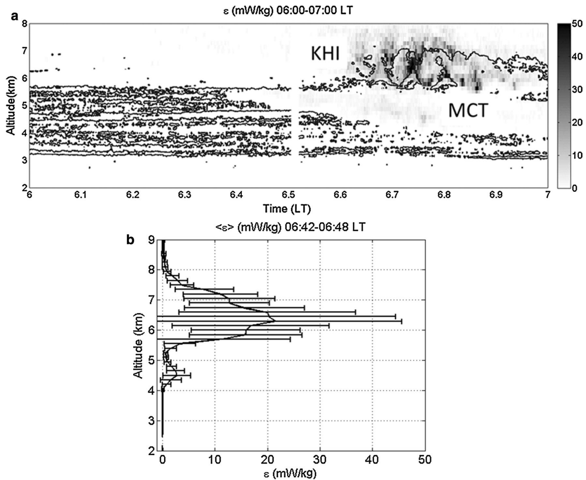
Fig. 9 a Turbulence kinetic energy dissipation rate \varepsilon (mWkg -1 ) between 0600 LT and 0700 LT. The black contours indicate an arbitrary level of the radar echo power. b Vertical profile of turbulence kinetic energy dissipation rate \varepsilon (mWkg -1 ) averaged over 6 min from 0642 LT to 0648 LT. The horizontal bars show the time variability ( \pm the standard deviation)
