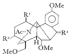
(422) : R 1 =R 2 =H, R 3 =O
