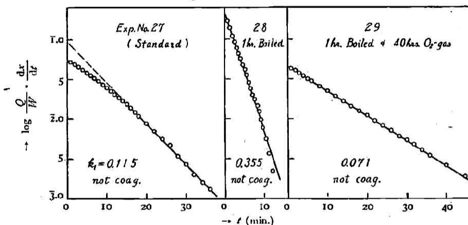
Fig. 7. The reactions with the boiled sol. (c). Initial conc. of \text{H}_2\text{O}_2 : 0.029 g.-mol./litre. Conc. of Pt-sol. (No. 5): 10 \times 10^{-6} g.-atom/litre. Temperature: 25°C.
