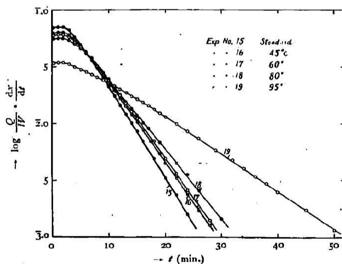
Fig. 5. The reactions with the heated sol.
