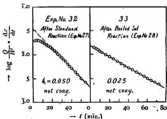
Fig. 9. The reactions with the sol once reacted. Initial conc. of \text{H}_2\text{O}_2 : 0.029 g.-mol./litre. Conc. of Pt-sol. (No. 5): 5 \times 10^{-6} g.-atom/litre. Temperature: 25^{\circ}\text{C}.
