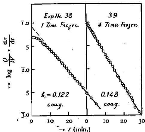
Fig. 11. The reactions with the frozen sol. ( -78^{\circ}\text{C} ).
