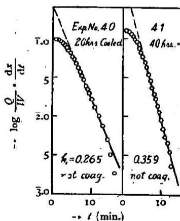
Fig. 12. The reactions with the cooled sol.
