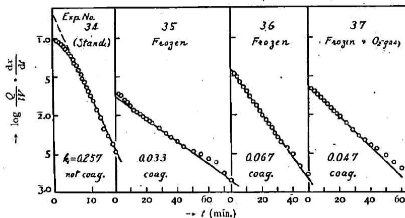
Fig. 10. The reactions with the frozen sol. ( -20^{\circ}\text{C} ).
