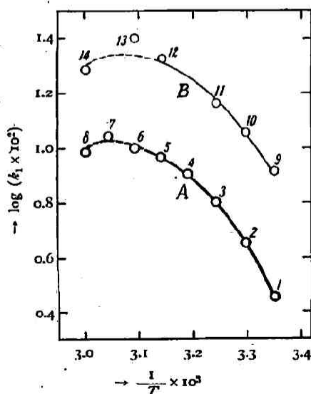
Fig. 3. Relation between the reaction velocity constant and temperature. Curve(A): Conc. of Pt-sol. 4 \times 10^{-6} g.-atom/litre. Curve(B): Conc. of Pt-sol. 8 \times 10^{-6} g.-atom/litre.
