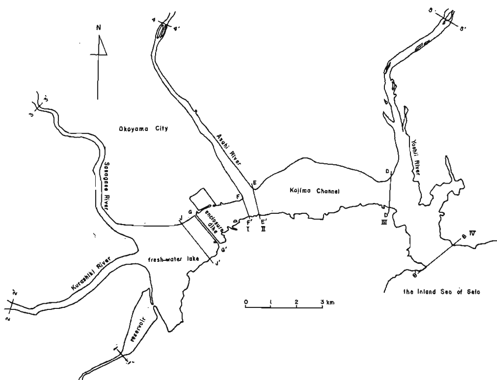
Fig. 7 Sounding lines for the survey of bottom topography—I, II, III, IV The limits of tidal effect —1, 2, 3, 4, 5
