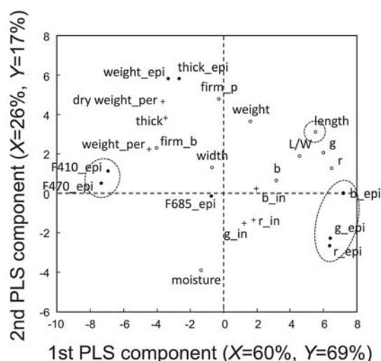
Fig. 6 PLS-DA loading plot. Component 1 vs. 2. The percentage in the axis shows the explanation power of each PLS component for the X- and Y-variables (24 traits and binary values of the groups ( -1 and 1 ), respectively). The positive value of the 1st loading is related with the dark group. The abbreviations F410, F470, and F685 stand for the fluorescence of the dried epidermis (epi) at 410, 470, and 685 nm, respectively (excitation at 365 nm). r, g, and b indicate the absorption of red, green, and blue light, respectively, at the fruit surface, inner (in) pericarp, and dried epidermis (epi). The other variables can be referred to in Table S1 in the ESI.† The open circle, cross, and filled circle indicate the traits of the fruit, pericarp, and epidermis, respectively.
