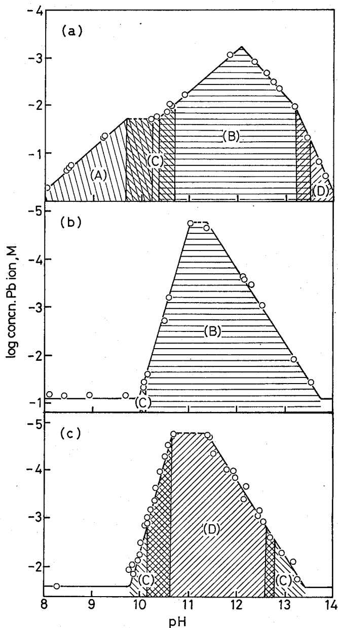
Fig. 3. Solubilities of lead compounds (A= \text{Pb}(\text{OAc})_2 \cdot 2\text{Pb}(\text{OH})_2 , B= \text{PbO} \cdot 2/5\text{H}_2\text{O} , C=orthorhombic \text{PbO} , D=tetragonal \text{PbO} ) at various pH values of the suspensions with 0.5(a), 0.008(b) and 0.025M \text{Pb}(\text{OAc})_2 (c) subjected to aging at 25^\circ\text{C} .
