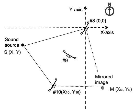
Fig. 6. Geometry of sound source and mirrored image localization. #8 (0, 0) and #10 ( X_{10} , Y_{10} ) are the positions of #8-AUSOMS-D and #10-AUSOMS-D. The position of the sound source is S(X, Y) and the position of the mirrored image is M(X_M, Y_M) . The sound source and the mirrored image are detected with two hydrophones at each of #8 (0, 0) and #10 ( X_{10} , Y_{10} ). The correct position of the sound source was determined as S(X, Y) by using the angle of \theta_9 .
