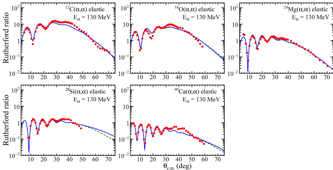
FIG. 5. Same as Fig. 4, but for ^{12}\text{C} , ^{16}\text{O} , ^{24}\text{Mg} , ^{28}\text{Si} , and ^{40}\text{Ca} at E_\alpha = 130 MeV.
