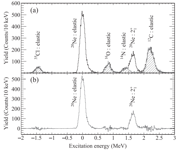
FIG. 2. Excitation-energy spectra for the ^{20}\text{Ne}(\alpha, \alpha') reaction at E_\alpha = 386 MeV measured at \theta_{\text{lab}} = 10.8^\circ . (a) The open histogram represents the excitation-energy spectrum obtained using the gas cell filled with ^{20}\text{Ne} . The hatched histogram represents the normalized spectrum obtained using the empty gas cell. (b) A background-free ^{20}\text{Ne}(\alpha, \alpha') spectrum obtained by subtracting the background events originated from aramid films.
