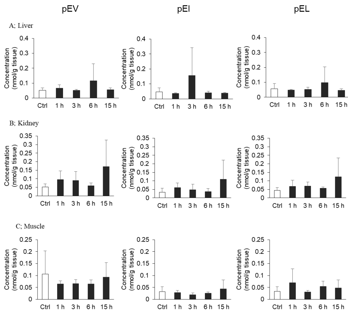
Figure 3-2. Contents of pyroglutamyl peptides after oral administration of mixture of pyroglutamyl peptides.
