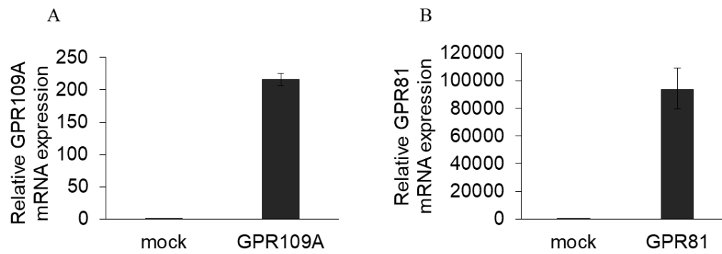
Figure 1-7. Expression of huGPR109A and huGPR81 in transfected NCM460D cell lines.
