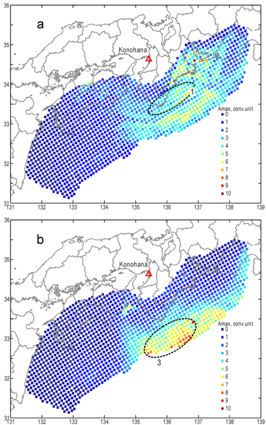
Fig. 9 Distribution of simulated peak GF amplitudes for velocity structure without sediment layers. a Transverse component for rake = 0^\circ and (b) radial component for rake = 90^\circ . Waveforms here and in Fig. 10 were simulated by FDM using the reciprocity method and the JIVSM velocity structure model, but with layers for which V_S < 2.4 km/s were replaced by layers with V_S = 2.4 km/s. S-wave velocity cross section is shown in Fig. 10. Other annotations as in Fig. 6
