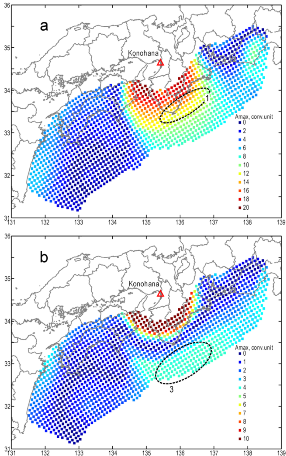
Fig. 6 Distribution of simulated peak GF amplitudes for subsources in an infinite uniform medium. a Transverse component for rake = 0° and (b) radial component for rake = 90°. Dashed ellipses indicate locations of anomalies 1 and 3 shown in Fig. 4
