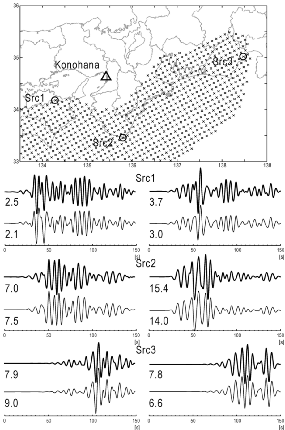
Fig. 3 Validation of the reciprocity approach. Comparison of reciprocal waveforms ( thick lines ) and forward simulated waveforms ( thin lines ) for EW ( left ) and NS ( right ) components for point sources Src1, Src2, and Src3, and for JIVSM model. Numbers at the left of each trace are normalized peak amplitudes
