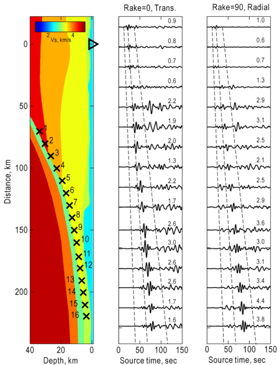
Fig. 10 Example of waveforms simulated with velocity structure without sediments. Cross section of S -wave velocity structure and location of subsources (left), transverse component waveforms for rake = 0° (center), and radial component for rake = 90° (right). Other annotations as in Fig. 5
