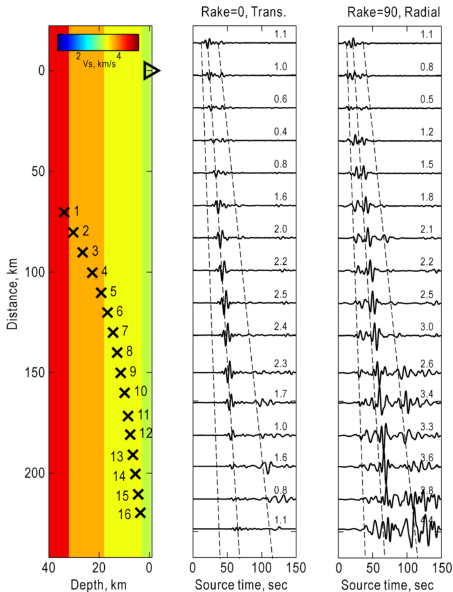
Fig. 8 Examples of simulated waveforms for 1D velocity structure along. Cross section of S -wave velocity structure and locations of subsources (left), waveform examples for transverse component for rake = 0^\circ (center) and for radial component for rake = 90^\circ (right). Other annotations as in Fig. 5
