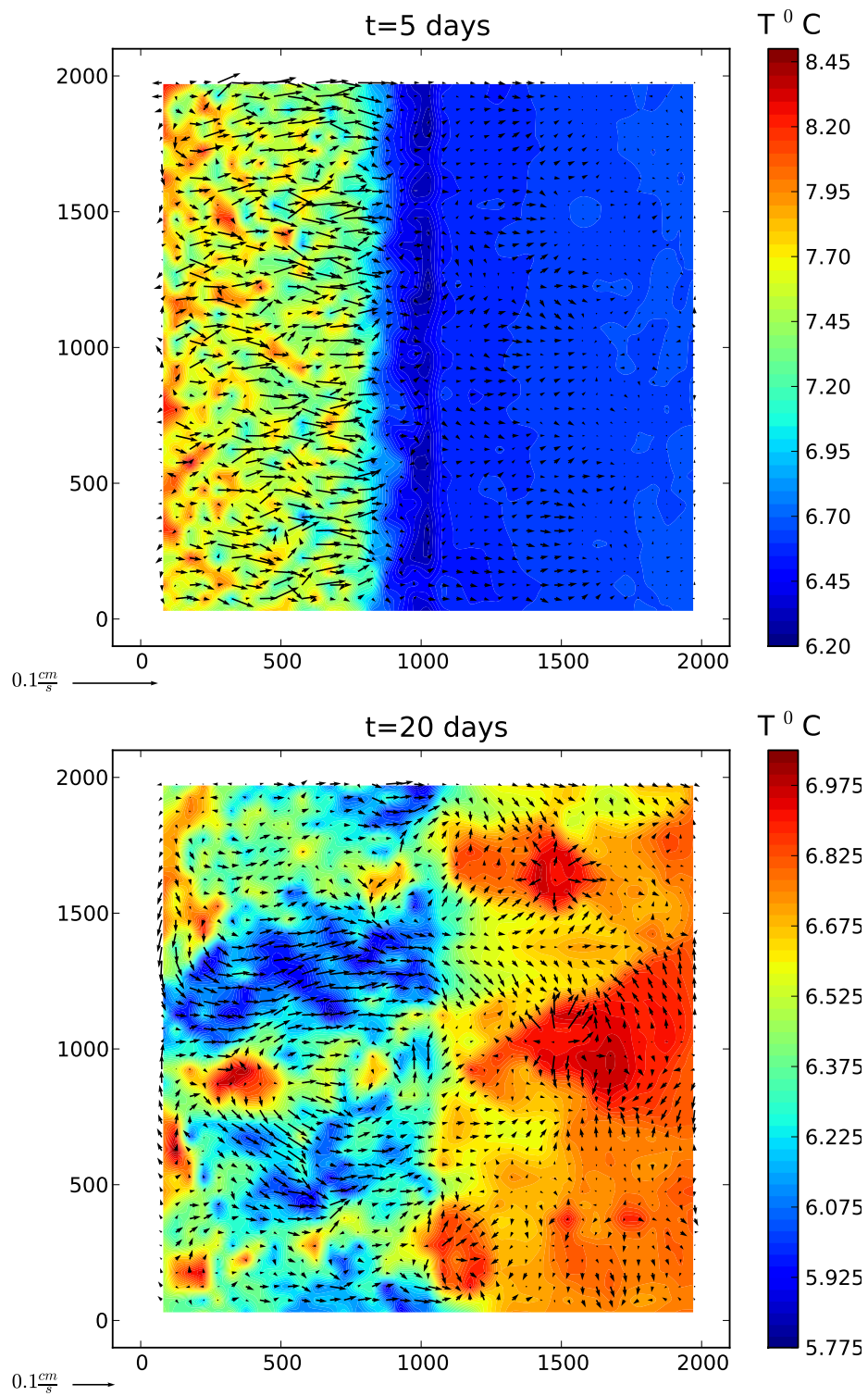
Figure 5.5: Plan view showing simulated flow from simulation with 8 % slope. Data are taken from cells adjacent to lake's bed or slope
