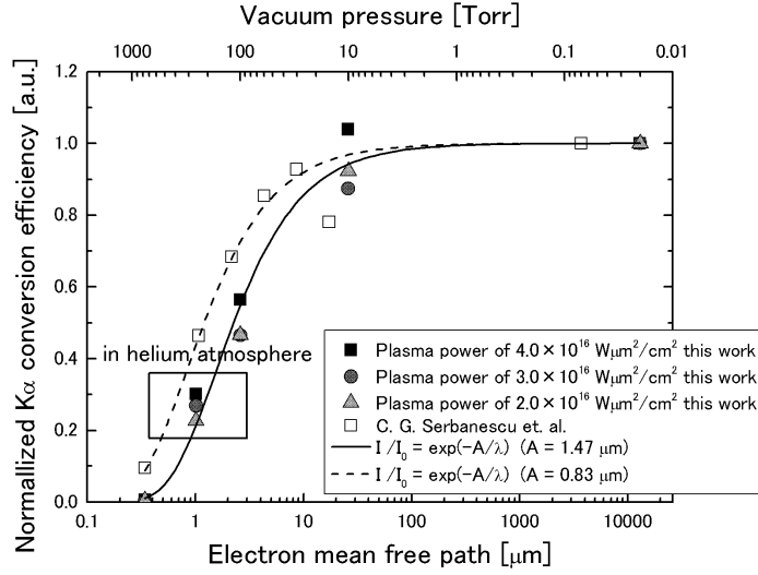
Figure 3.11: Comparison between the normalized K\alpha X-ray conversion efficiency in this work and in Serbanescu et. al.. Symbols are indicated in the inset legend.
