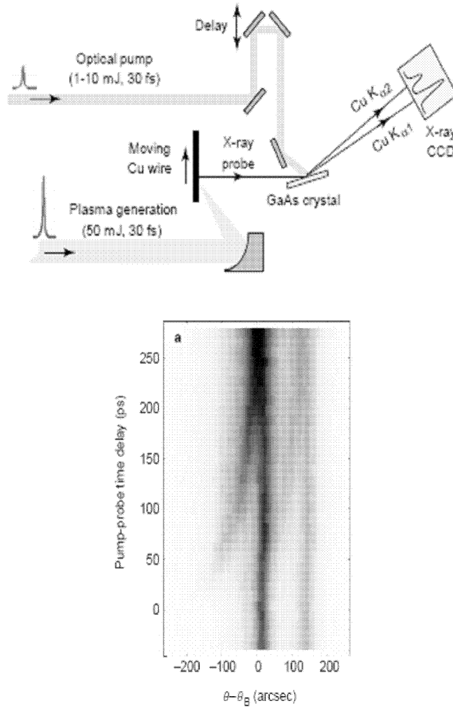
Figure 1.3: Acoustic coherent phonon in a semiconductor observed with the time-resolved X-ray diffraction method. (C. Rose-Petruck et al. 20) )
