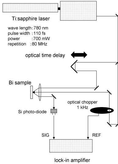
Figure 2.12: The experimental setup for pump-probe measurements of optically induced reflectivity changes.
