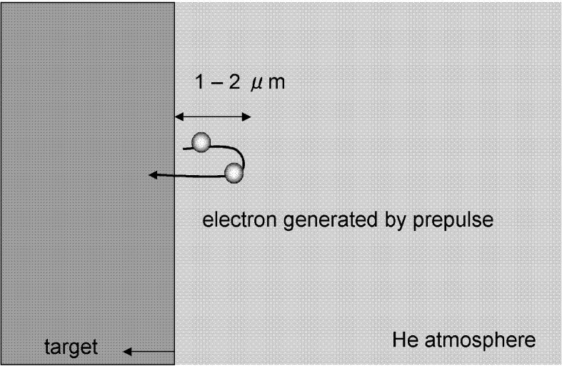
Figure 3.16: The effect of the prepulse considered based on the simple electron collision model.
