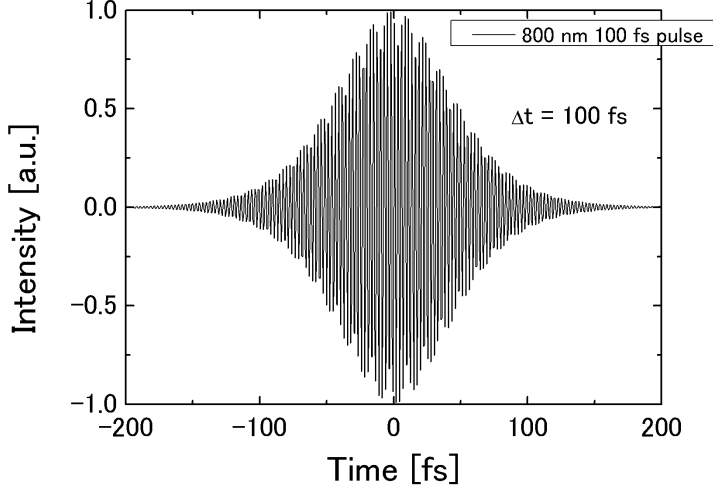
Figure 2.8: A femtosecond laser pulse described as the function of \text{sech}^2(t)
