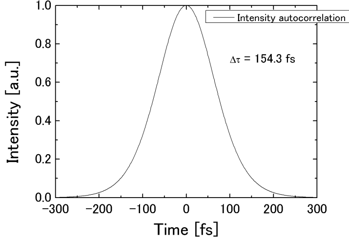
Figure 2.9: The autocorrelation function of a femtosecond laser pulse at the pulse duration of 100 fs.
