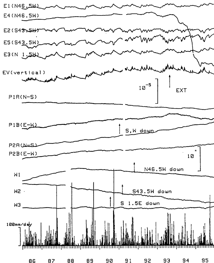
Fig. 1 Secular variations of ground-strains observed with extensometers (E1~5, EV) ground-tilts observed with horizontal pendulum tiltmeter pairs (P1, P2), water-tube tiltmeters (W1 ~ W3) and precipitation at the Miyazaki Observatory.
