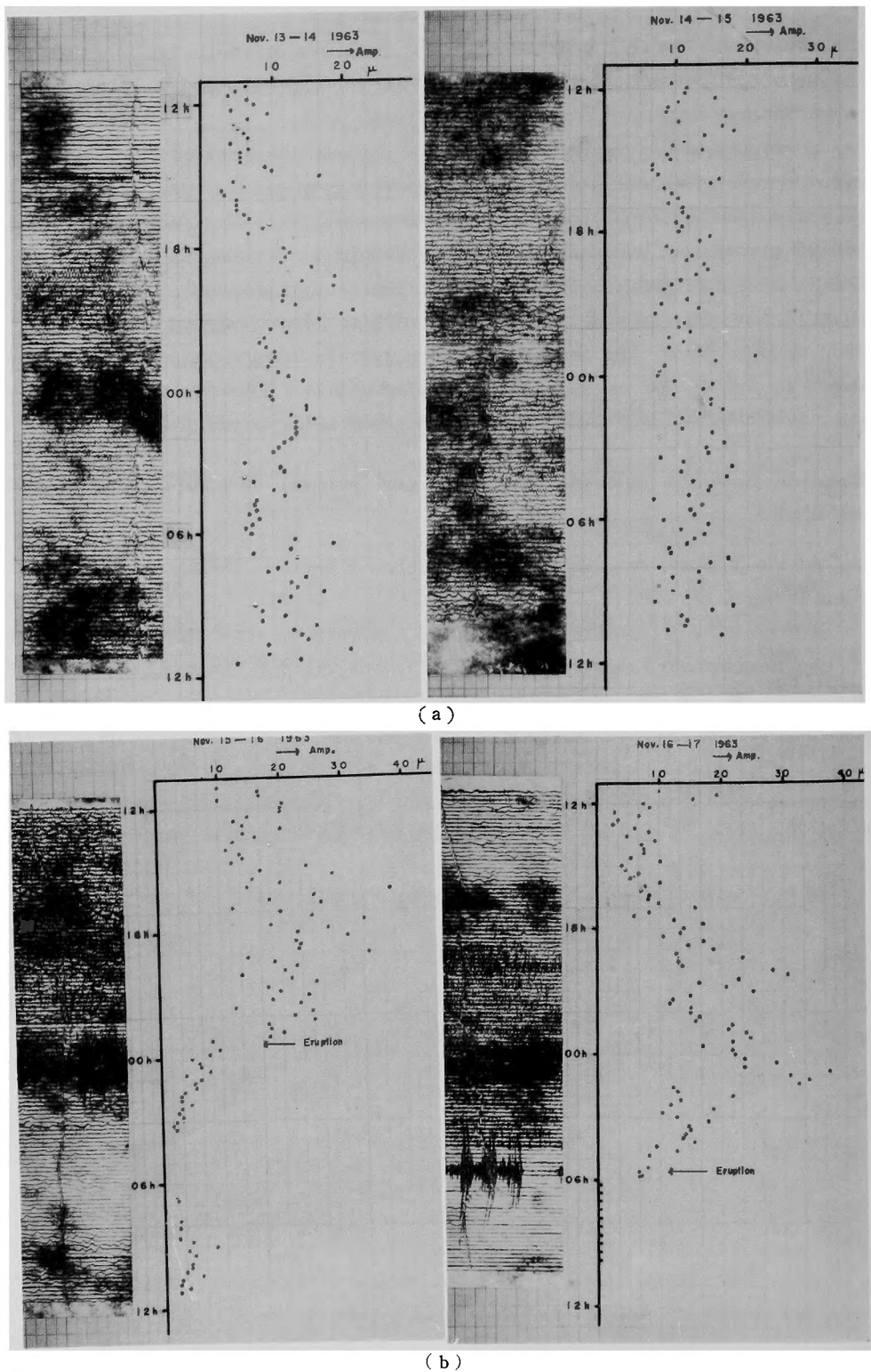
Fig. 10. Peculiar variation of amplitude of the 3rd-kind volcanic micro tremor before the eruption on Nov. 17, 1963.
