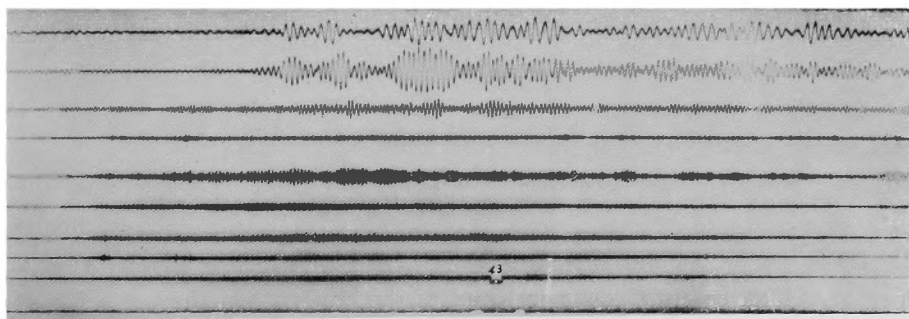
Fig. 6. The frequency analysed record of Northern Celebes Earthquake.
