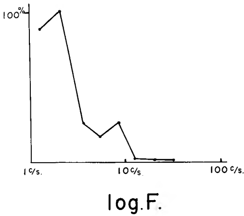
Fig. 4. Displacement-amplitude vs. frequency curve of Fig. 3.
