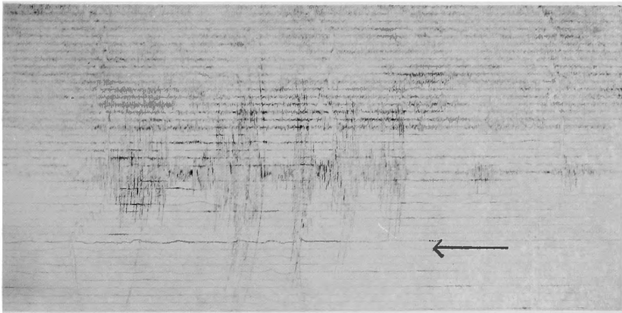
Fig. 9. Seismic record of the small eruption on Nov. 17, 1963.
