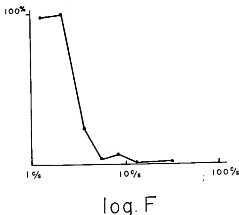
Fig. 7. Displacement-amplitude vs. frequency curve of Fig. 6.
