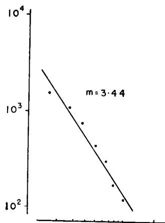
Fig. 8. Annual amplitude distributions of the 3rd-kind volcanic micro tremor.
