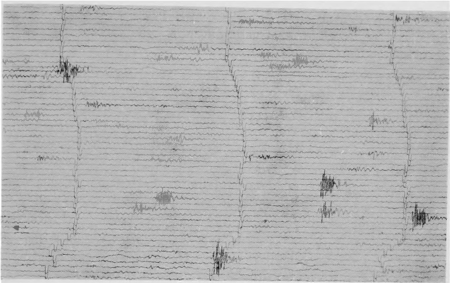
Fig. 1. Seismic record of the 3rd-kind volcanic micro tremor when it appears in the form of isolated waves.
