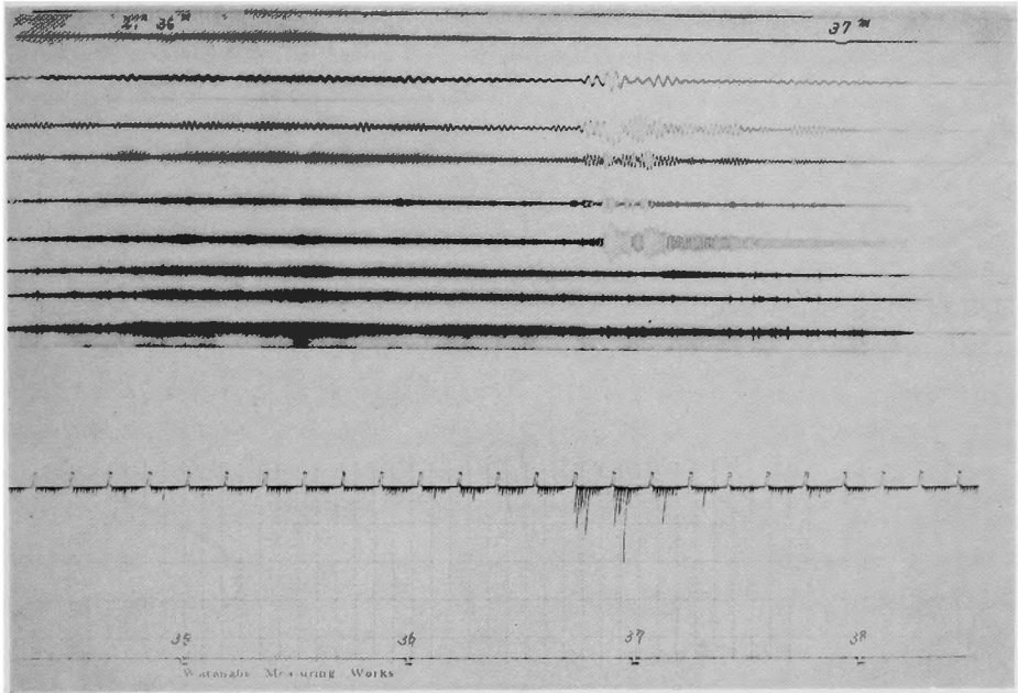
Fig. 3. Frequency analysed record of the 3rd-kind volcanic micro tremor.
