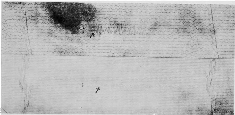
Fig. 2. Simultaneous records of the 3rd-kind volcanic micro tremor. Upper part : Hondō Lower part : Laboratory
