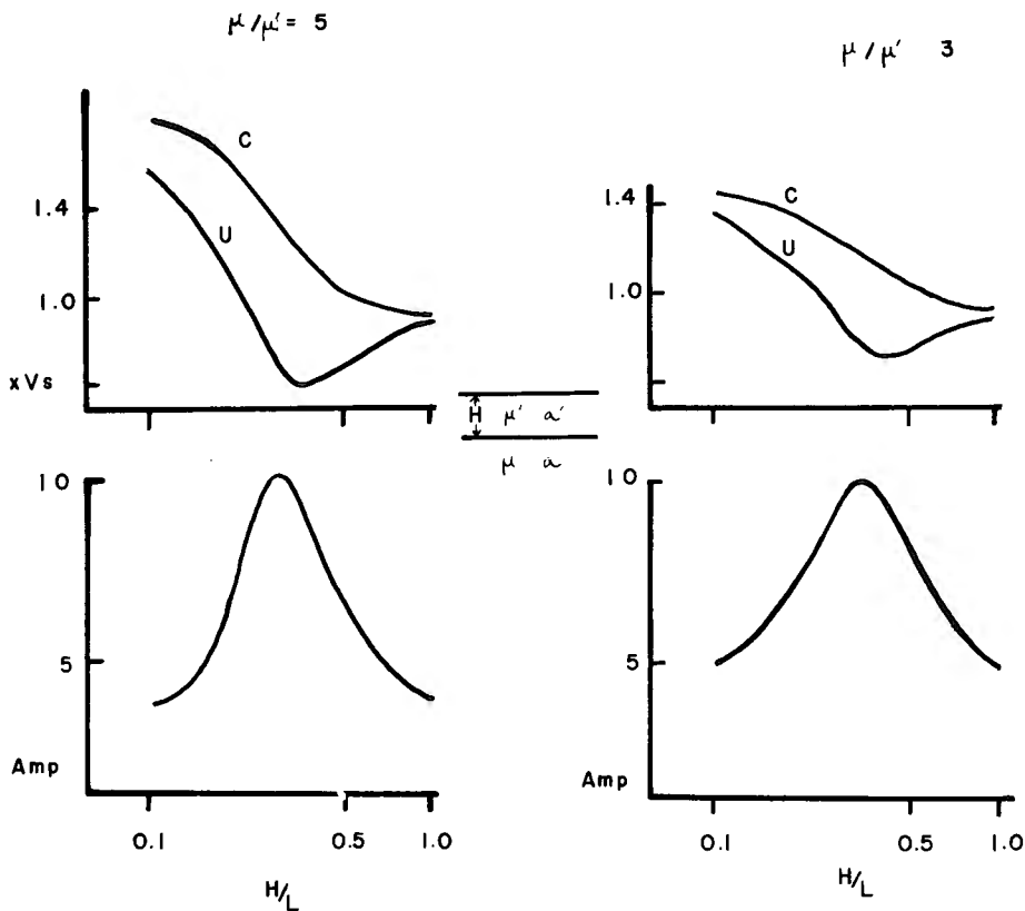
Fig. 5. Phase- and group-velocity and amplitude vs. H/L curves of the Rayleigh wave in a solid layer over solid half space. (after Y. Oota)
