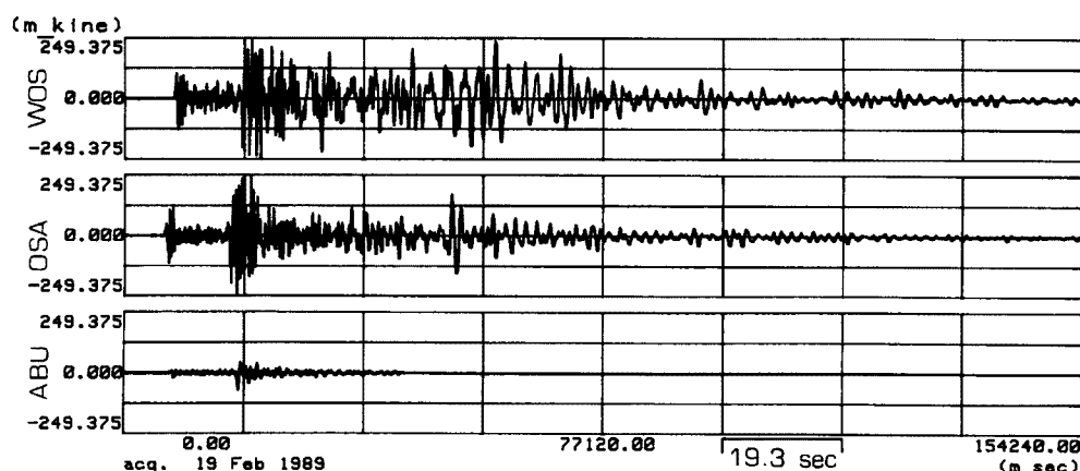
Fig. 7. Comparison of wave forms observed at WOS, OSA and ABU for the earthquake (1989 Feb. 19, M=5.3 , H=52 km) in the central part of the Mie prefecture. Traces are vertical components of particle velocity.
