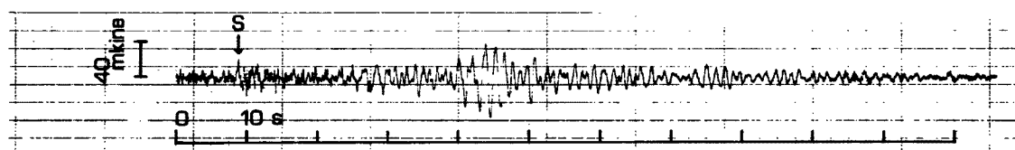
Fig. 8. Wave form observed at OSA for the earthquake (1989 May 2, M=4.1 , H=32 km) near Shiga-Gifu border. Trace is a vertical component of particle velocity.
