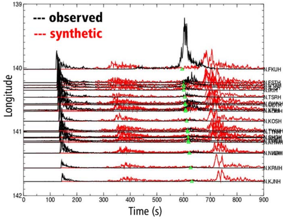
Fig. 11 Envelopes of the Hi-net UD components filtered at 2–5 Hz (in black) and synthetic envelopes from the FDM simulation (in red). Green triangles show the theoretical arrival time of the T-phase.
