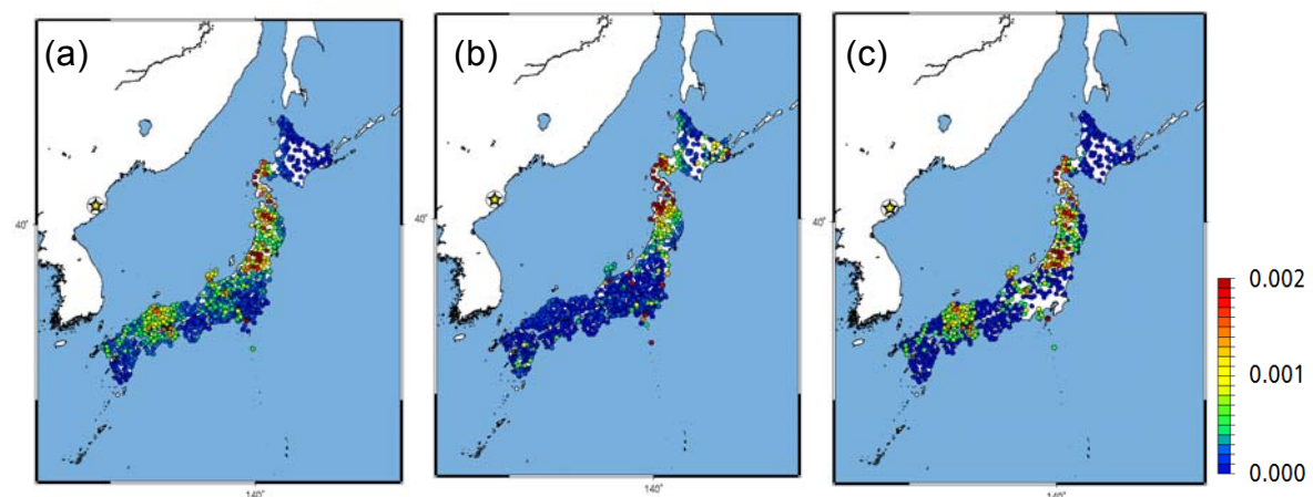
Fig. 2 Amplitudes recorded at Hi-net seismic station. UD component filtered at 2–5 Hz in cm/s. (a) Nuclear explosion in 2017, (b) T-phase, and (c) Earthquake in 2002.
