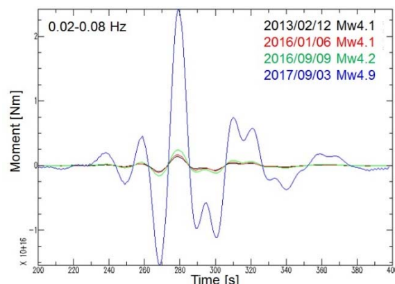
Fig. 6 Estimated isotropic sources of the past nuclear tests
