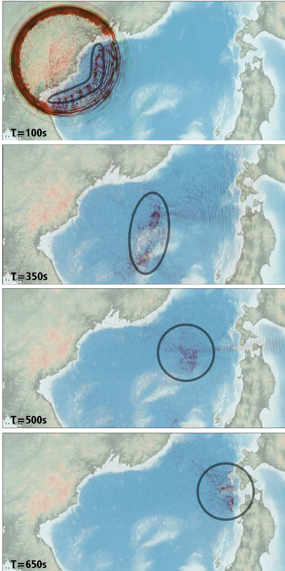
Fig. 10 Ground motion simulation at T=100s , 350s , 500s , and 650s from the origin time. Green and red colors show the horizontal and vertical waves at the ocean bottom. Gray circles indicate the T-phase.
