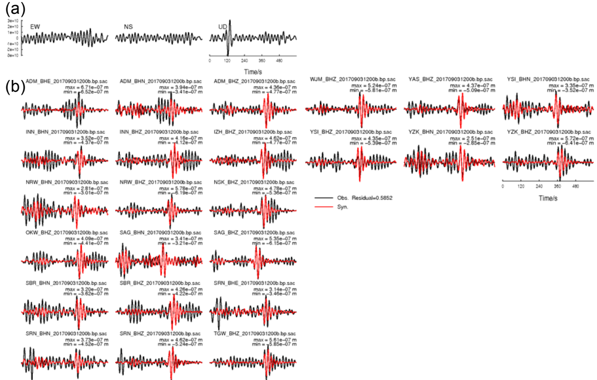
Fig. 8 (a) Estimated single forces at the source and (b) observed (in black) and synthetic (in red) waveforms.
