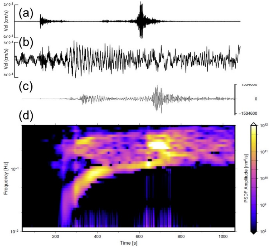
Fig. 12 Waveforms at N.FKUH station (a) observation at 2–5 Hz (b) observation at 0.02–0.5 Hz (c) simulation (d) spectrogram of the simulation
