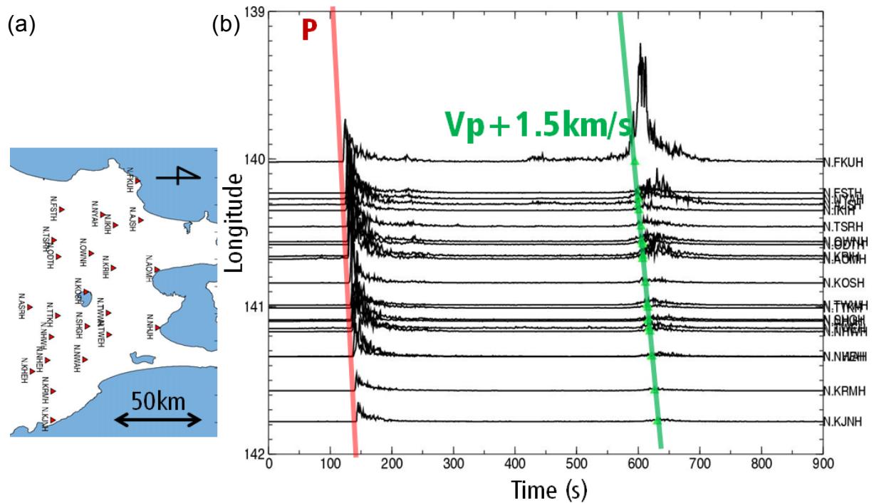
Fig. 9 (a) Station map and (b) envelopes of the Hi-net UD components filtered at 2–5 Hz.
