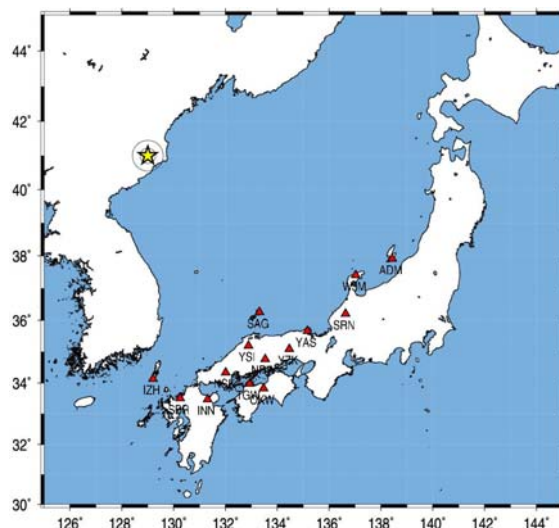
Fig. 7 Stations used for the waveform inversion of the collapse shown in red triangles. The yellow star shows the source location.
