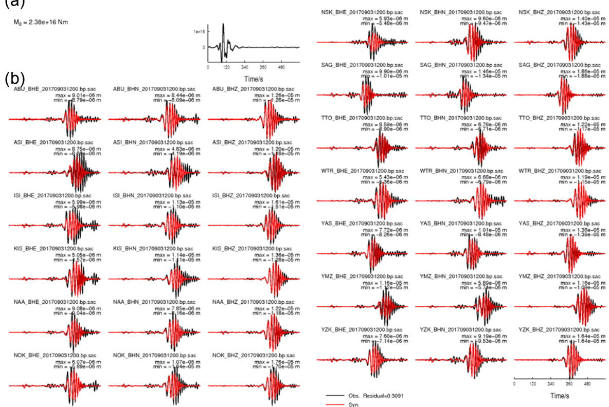
Fig. 5 (a) Estimated isotropic source at 0.02–0.08 Hz and (b) observed (in black) and synthetic (in red) waveforms.
