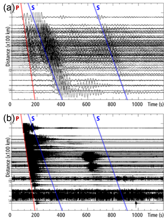
Fig. 1 F-net waveforms (a) 0.02–0.05 Hz and (b) 2–5 Hz
