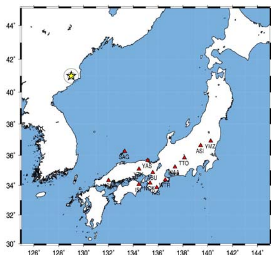
Fig. 4 Stations used for the waveform inversion of the nuclear explosion shown in red triangles. The yellow star shows the source location.
