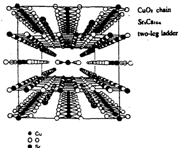
図1 \text{Sr}_x\text{Ca}_{14-x}\text{Cu}_{24}\text{O}_{41} の結晶構造
