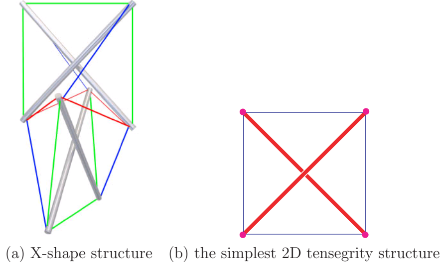
Figure 1.3: The X-shape tensegrity structure in (a), courtesy of K. Snelson and http://www.kennethsnelson.net , is an assemble of the two-dimensional modules in (b), one to the other. The picture is a reproduction of X-shape tensegrity structure created by Snelson in 1948.
