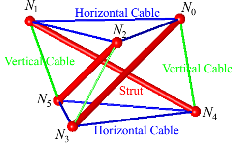
Figure 1.1: The simplest tensegrity structure in three-dimensional space. Struts are denoted by thick lines and cables by thin lines. A class of structures similar to this one will be revisited in Chapters 6 and 7 for their self-equilibrated configurations and stability properties.
