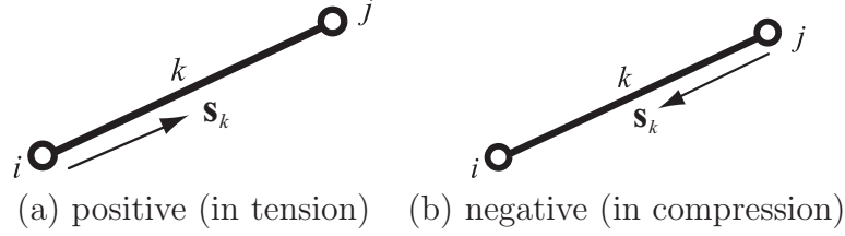
Figure 5.3: Definition of prestress vector \mathbf{s}_k ( i < j ). A cable that is in tension is defined to have positive direction pointing from one of its node bearing smaller number to the other node with larger number, and a strut that is in compression has negative direction.
