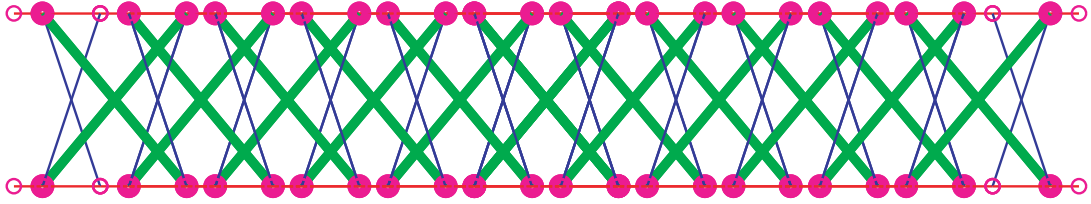
Figure 11.5: Example 1: self-equilibrated configuration of the structure when force density of the horizontal cable is given as q_{h_2} = 2 .
