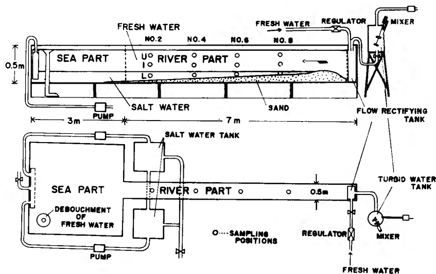
Fig. 1. Experimental flume.
