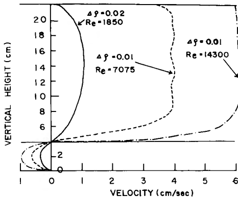
Fig. 3. Vertical distribution of velocity before discharge of turbid water.
