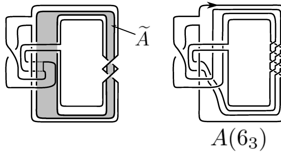
Figure 4: A shrunken annulus \tilde{A} for the annulus presentation of 6_3 (left) and the knot A(6_3) (right).
