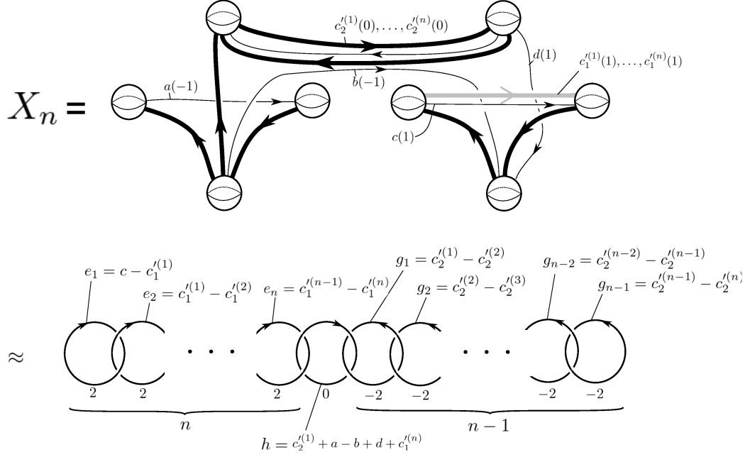
Figure 12: A Kirby diagram of X_n . The bold arc represents the parallel copies c'_2(1), \dots, c'_2(n) of c'_2 and the gray arc represents the parallel copies c'_1(1), \dots, c'_1(n) of c'_1 . In the top picture, the number in “( )” on the right of each curve represents the framing. The bottom picture is obtained from the top by Kirby calculus as in the pictures depicted in the end of this manuscript. The bottom picture is a framed link with 2n components and the numbers 2, 2, \dots, 2, 0, -2, -2, \dots, -2, -2 represent the framing.
