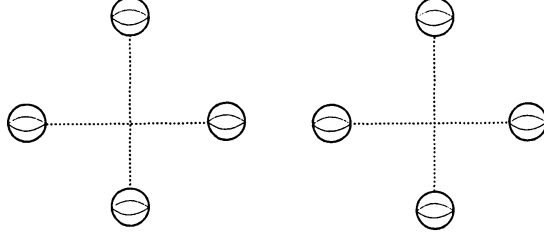
Figure 11: The trivial D^2 -bundle over \Sigma_{2,1} .
