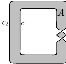
Figure 2: An unknotted annulus A \subset S^3 with a +1 full-twist.
