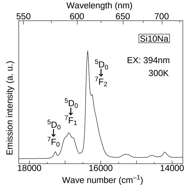
Fig. 3.1. Fluorescence spectra of \text{Eu}^{3+} in 90\text{SiO}_2 \cdot 10\text{Na}_2\text{O} \cdot 1\text{Eu}_2\text{O}_3 glass at room temperature excited by broadband excitation (Xe lamp) whose wavelength is 394 nm.
