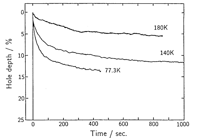
Fig. 6.7. The burning time dependence of the persistent hole depth for AH4 obtained by monitoring the ^5\text{D}_0 \rightarrow ^7\text{F}_2 emission in the presence of burning irradiation of a DCM dye laser of 681.8 nm.
