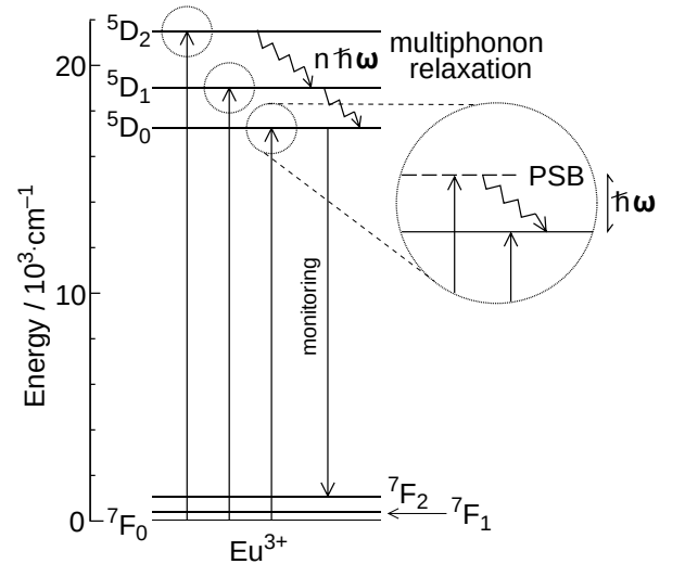
Fig. 1.2. A schematic diagram of phonon sideband process.
