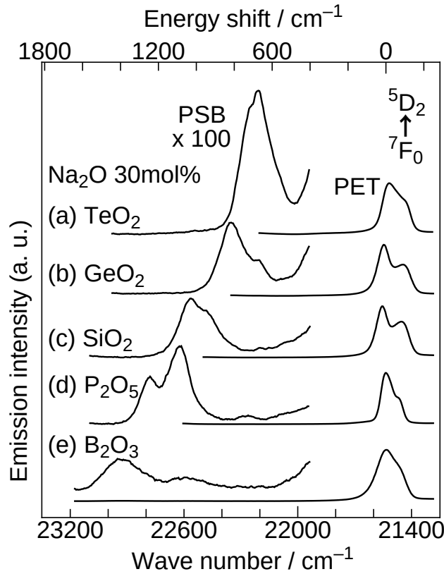
Fig. 1.1. Excitation spectra of {}^5\text{D}_0 \rightarrow {}^7\text{F}_2 emission of \text{Eu}^{3+} doped in 70\text{M}_x\text{O}_y \cdot 30\text{Na}_2\text{O} glasses at room temperature. Phonon sideband (PSB) associated with the {}^5\text{D}_2 \leftarrow {}^7\text{F}_0 transition appears at higher energy side. The energy gap between PSB and pure electronic transition (PET) corresponds to phonon energy, \hbar\omega , due to the lattice vibration around \text{Eu}^{3+} ions.
