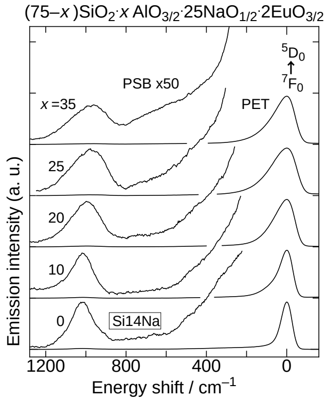
Fig. 1.7. Phonon sideband spectra associated with ^5D_0 \leftarrow ^7F_0 transition of \text{Eu}^{3+} in sodium aluminosilicate glasses at 10 K by monitoring ^5D_0 \rightarrow ^7F_2 emission at 612 nm.
