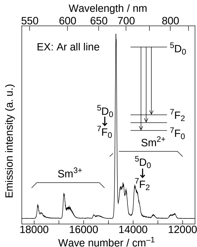
Fig. 6.3. Fluorescence spectrum at 4.5 K of AH4 under excitation by \text{Ar}^+ ion laser (all line) and energy diagram of \text{Sm}^{2+} .
