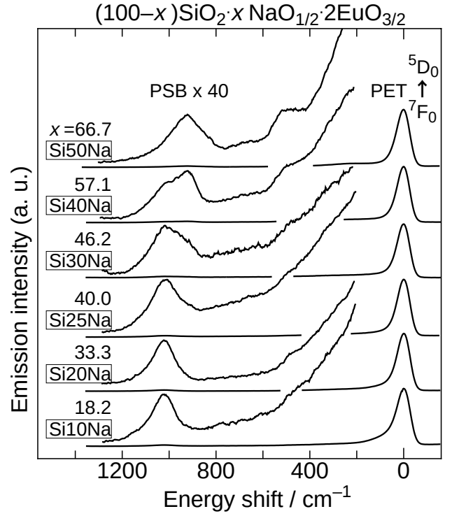
Fig. 1.5. Phonon sideband spectra associated with ^5D_0 \leftarrow ^7F_0 transition of \text{Eu}^{3+} in sodium silicate glasses at 10 K by monitoring ^5D_0 \rightarrow ^7F_2 emission at 612 nm.
