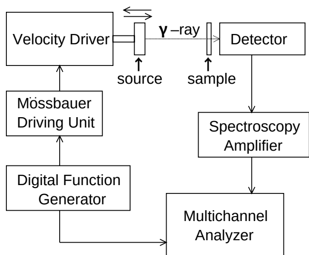
Fig. 2.1. Schematic diagram of the experimental setup for Mössbauer spectroscopy.
