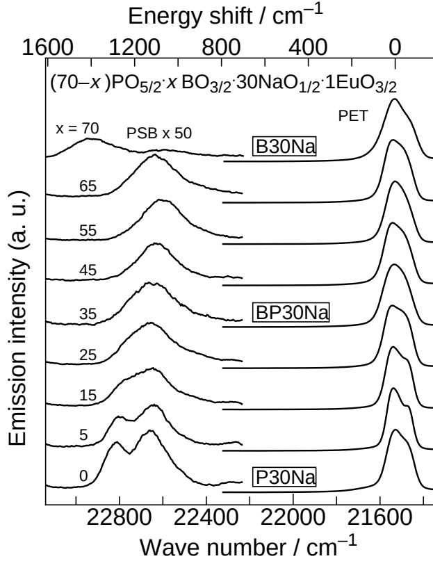
Fig. 4.5. Phonon sideband spectra associated with ^5D_2 \leftarrow ^7F_0 transition of \text{Eu}^{3+} in sodium borophosphate glasses (B-P system) at room temperature by monitoring ^5D_0 \rightarrow ^7F_2 emission at 612 nm.
