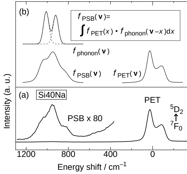
Fig. 1.3. (a) Phonon sideband spectrum associated with ^5D_2 \leftarrow ^7F_0 transition of \text{Eu}^{3+} in Si40Na glass at room temperature and (b) the diagram showing calculation of PSB curve, f_{\text{PSB}}(\nu) , from the PET curve, f_{\text{PET}}(\nu) , and the phonon distribution curve, f_{\text{phonon}}(\nu) .
