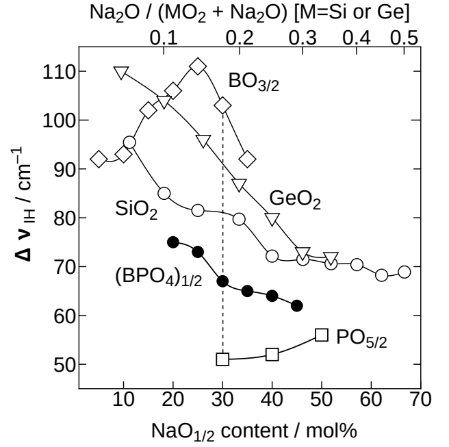
Fig. 4.3. Compositional dependence of the linewidth of the {}^5D_0 \rightarrow {}^7F_0 transition of \text{Eu}^{3+} , \Delta\nu_{1H} , in several oxide glasses. The dashed line represents B-P system.
