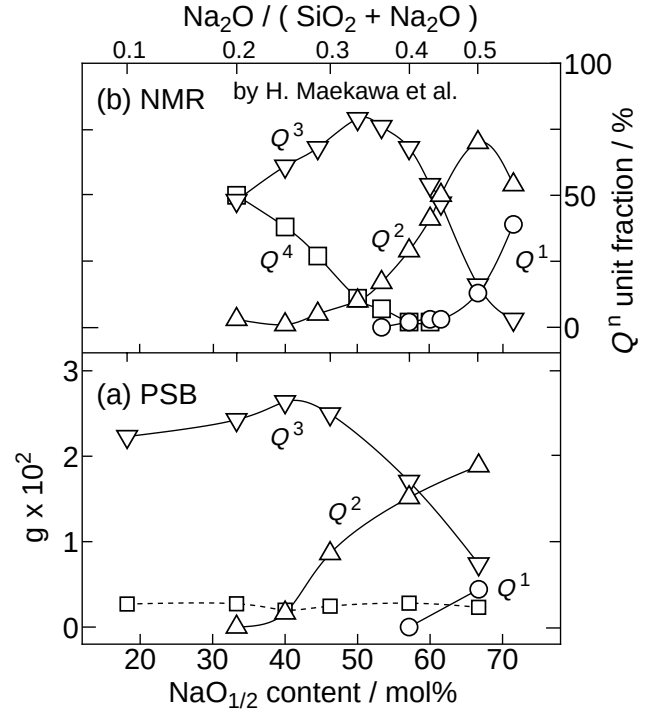
Fig. 1.10. Compositional dependence of the amount of Q^n units (a) in the local structure around \text{Eu}^{3+} ions (this study) and (b) in rare earth-free sodium silicate glasses investigated by Maekawa et al. using ^{29}\text{Si} MAS-NMR[53]. The vertical axes are taken as (a) an intensity ratio of the peak to PET peak, g , and (b) the fraction of Q^n unit. \square is the same as Fig. 1.9. (b) is reproduced using the Tables 1 and 2 in [53].
