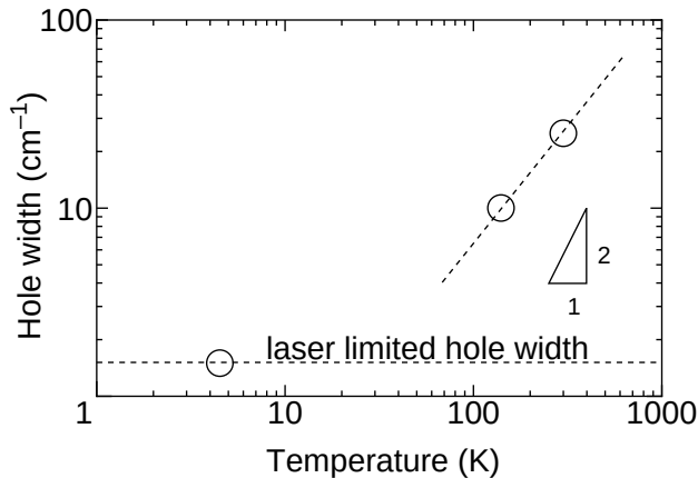
Fig. 6.6. Temperature dependence of the hole width.
