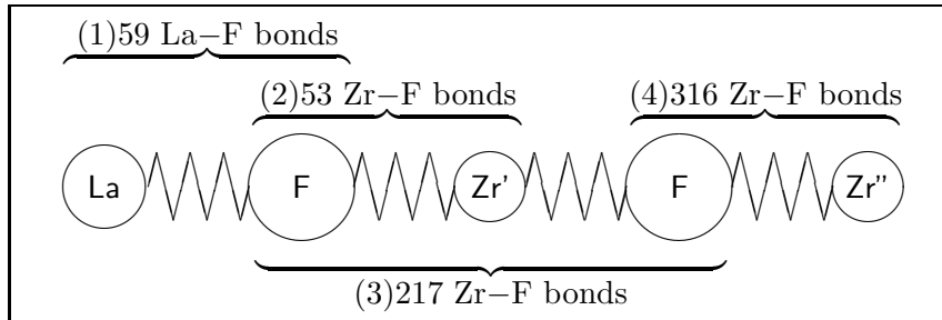
Fig. 5.8. The four groups of bonds in the MD-simulated glass. \text{Zr}' : within the second coordination shell of La ions, \text{Zr}'' : out of the second coordination shell of La ions. (1) La-F, (2) Zr-F surrounding La ions, (3) Zr-F within the third coordination shell, and (4) Zr-F out of the second coordination shell.
