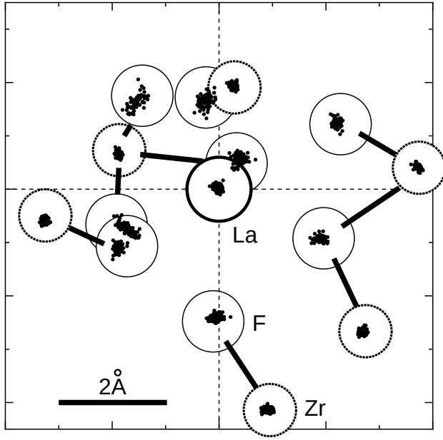
Fig. 5.7. Snapshot of the local structure within the second coordination sphere of \text{La}^{3+} ion (within 5 Å) at 300 K. The trajectories of the atoms for 1000step (2 psec) are also shown.
