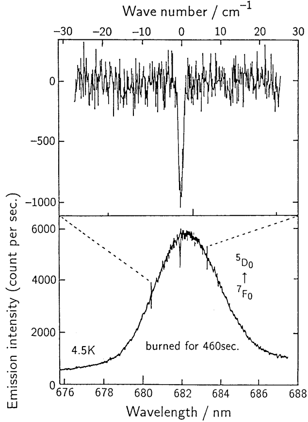
Fig. 6.4. Bottom: Excitation spectrum at 4.5 K of AH4 obtained by monitoring the ^5D_0 \rightarrow ^7F_2 emission before and after irradiation with a DCM dye laser of 681.8 nm. Burning time is 460 sec. Top: The difference signal at 4.5 K, magnified by a factor of 2.
