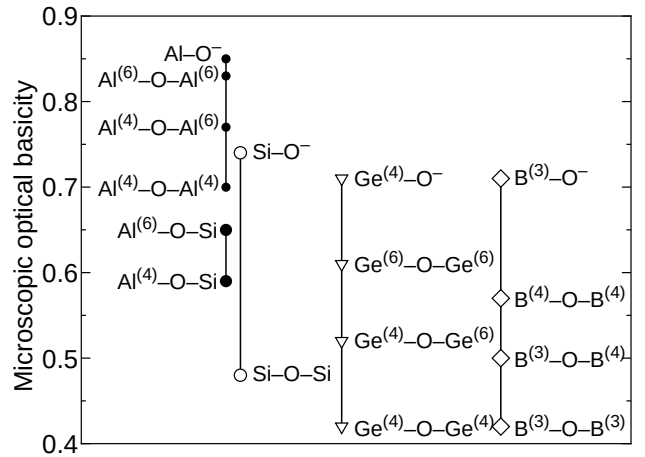
Fig. 2.5. The value of microscopic optical basicity, \lambda_{\text{th}} , for oxygen species that may be present in oxide glasses in this study. Numerals in parenthesis indicate the coordination number. See Appendix 2-A for detailed calculation.
