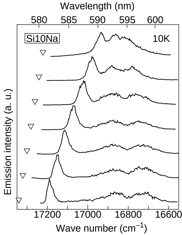
Fig. 3.5. Time-resolved site-selective fluorescence spectra of the ^5D_0 \rightarrow ^7F_1 transition of \text{Eu}^{3+} in (a) 81.8\text{SiO}_2 \cdot 18.2\text{NaO}_{1/2} glass (Si10Na) excited by various energies (denoted by triangles) and (b) borate glasses excited at 17322 \text{ cm}^{-1} . The fluorescence was measured at 10 K and at a delay of 0.2 msec after the laser pulse. The spectra are normalized to the same height.
