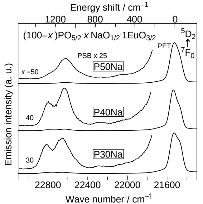
Fig. 4.4. Phonon sideband spectra associated with {}^5D_2 \leftarrow {}^7F_0 transition of \text{Eu}^{3+} in sodium phosphate glasses at room temperature by monitoring {}^5D_0 \rightarrow {}^7F_2 emission at 612 nm.
