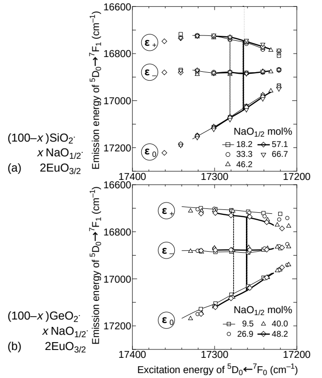
Fig. 3.6. Variation of the splitting of ^5D_0 \rightarrow ^7F_1 transition peak ( \epsilon_+ , \epsilon_- , and \epsilon_0 ) as a function of excitation energy for (a) silicate, (b) germanate, (c) aluminosilicate and (d) borate glasses. Errors are estimated to be equivalent to the size of each symbol. The tie lines represent the fluorescence peak profiles of the ^5D_0 \rightarrow ^7F_0 transition and the vertical lines their peak position (See Figs. 3.4(a)–3.4(d)).
