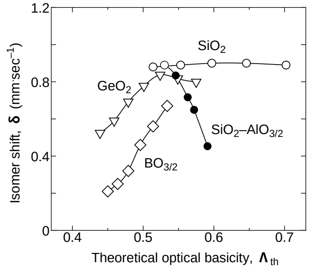
Fig. 2.4. Relationship between the isomer shift of ^{151}\text{Eu}^{3+} and the theoretical optical basicity, \Lambda_{\text{th}} , of the host glass.
