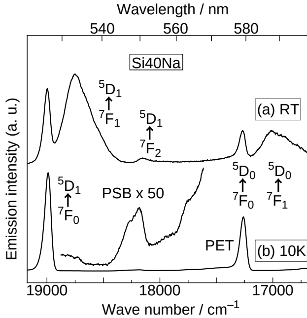
Fig. 1.4. Phonon sideband spectrum associated with ^5D_0 \leftarrow ^7F_0 transition of \text{Eu}^{3+} in 60SiO 2 ·40Na 2 O·1Eu 2 O 3 glass at (a) room temperature and (b) 10 K by monitoring ^5D_0 \rightarrow ^7F_2 emission at 612 nm.
