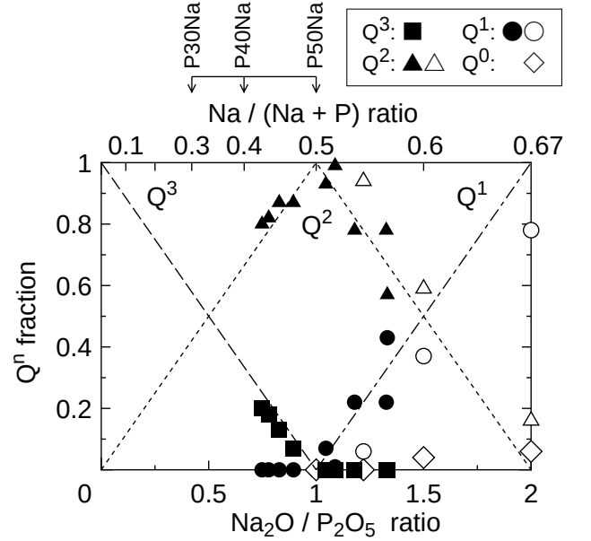
Fig. 4.1. Compositional dependence of the fraction of Q^n sites in M_2O+H_2O+P_2O_5 ( M : alkali metal) glasses as determined by ^{31}\text{P} MAS-NMR (solid symbols, Brow et al. [84]) and Raman spectroscopy (open symbols, Tatsumisago et al. [85]). The lines represent the calculated fractions based on the assumption that the equilibrium constants of the following equations are zero, i.e., the reactions go on the right side.
