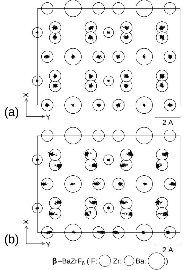
Fig. 5.11. The trajectories of ions in MD-simulated \text{BaZrF}_6 crystal during 1000 steps at intervals of 5 steps using (a) proper and (b) wrong potential parameters.
