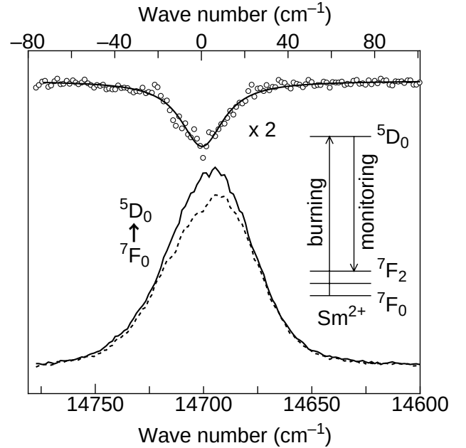
Fig. 6.5. Bottom: Excitation spectrum at room temperature of HBLAN obtained by monitoring the ^5D_0 \rightarrow ^7F_2 emission before and after irradiation with a DCM dye laser of 681 nm. Burning time is 900 sec. Top: The difference signal, magnified by a factor of 2.
