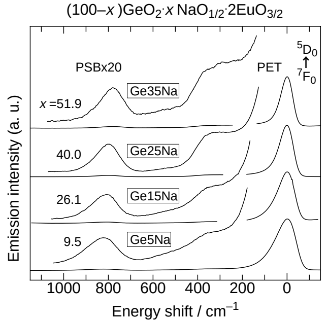
Fig. 1.6. Phonon sideband spectra associated with ^5D_0 \leftarrow ^7F_0 transition of \text{Eu}^{3+} in sodium germanate glasses at 10 K by monitoring ^5D_0 \rightarrow ^7F_2 emission at 612 nm.
