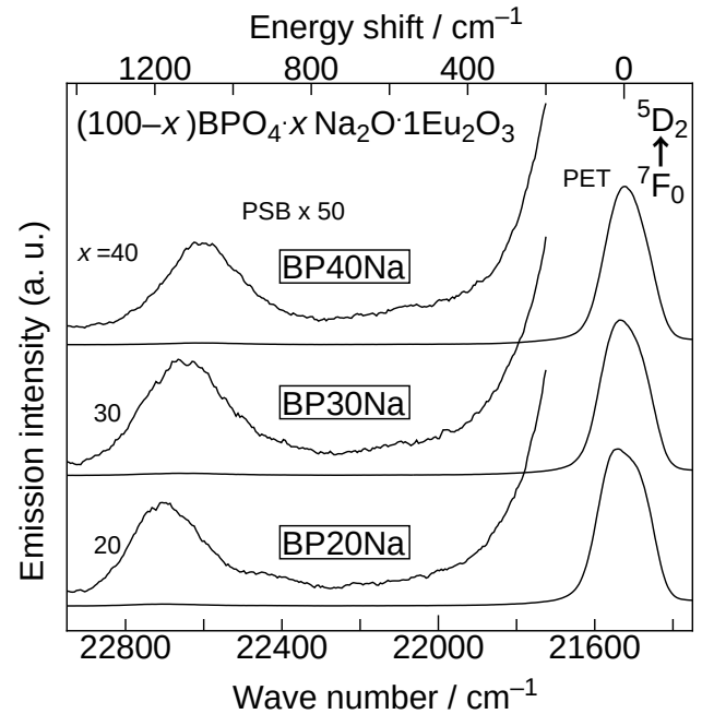
Fig. 4.6. Phonon sideband spectra associated with ^5D_2 \leftarrow ^7F_0 transition of \text{Eu}^{3+} in sodium borophosphate glasses (Na system) at room temperature by monitoring ^5D_0 \rightarrow ^7F_2 emission at 612 nm.
