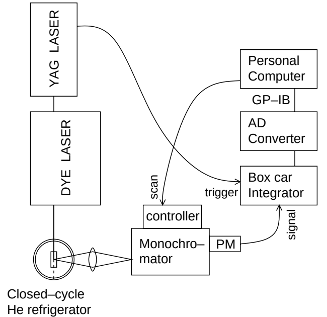
Fig. 3.3. Schematic diagram of the experimental setup for the time-resolved FLN measurement. PM: photomultiplier.
