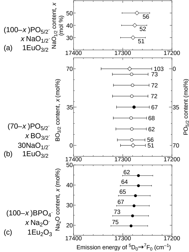
Fig. 4.2. Peak position of the {}^5D_0 \rightarrow {}^7F_0 transition of \text{Eu}^{3+} for (a) phosphate glasses, (b) B-P system, and (c) Na system. The length of the bar represents the full width at half-maximum, \Delta\nu_{1H} , numerals on the bar are the value of \Delta\nu_{1H} in \text{cm}^{-1} and the symbols on the bar correspond to the top position of peak. Errors were estimated as \pm 5 \text{ cm}^{-1} .
