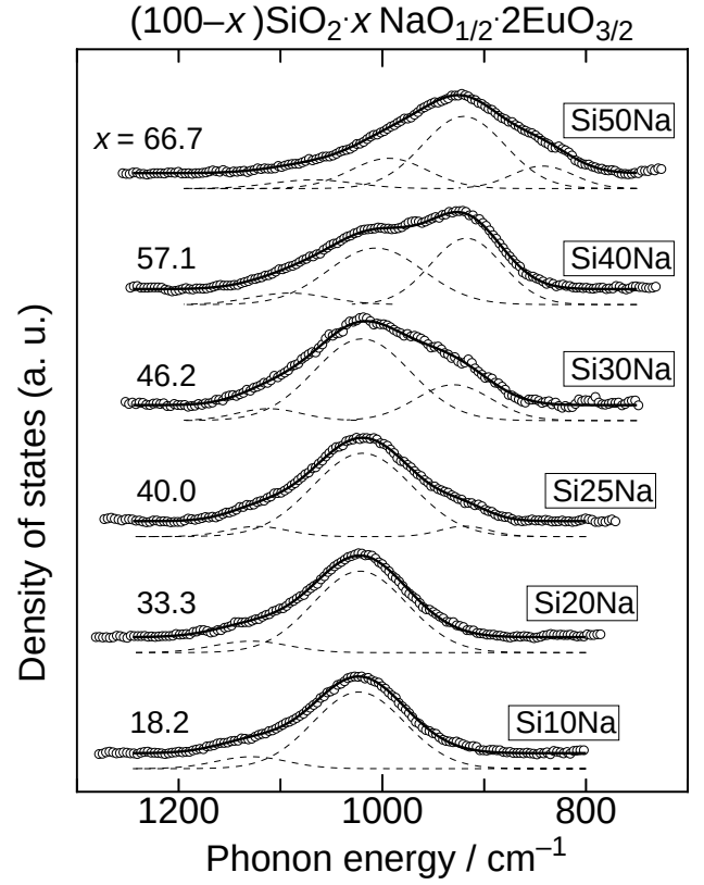
Fig. 1.8. Deconvolution of the PSB spectra for sodium silicate glasses. \circ : experimental data, - - -: Gaussian component, and —: sum of all the component.
