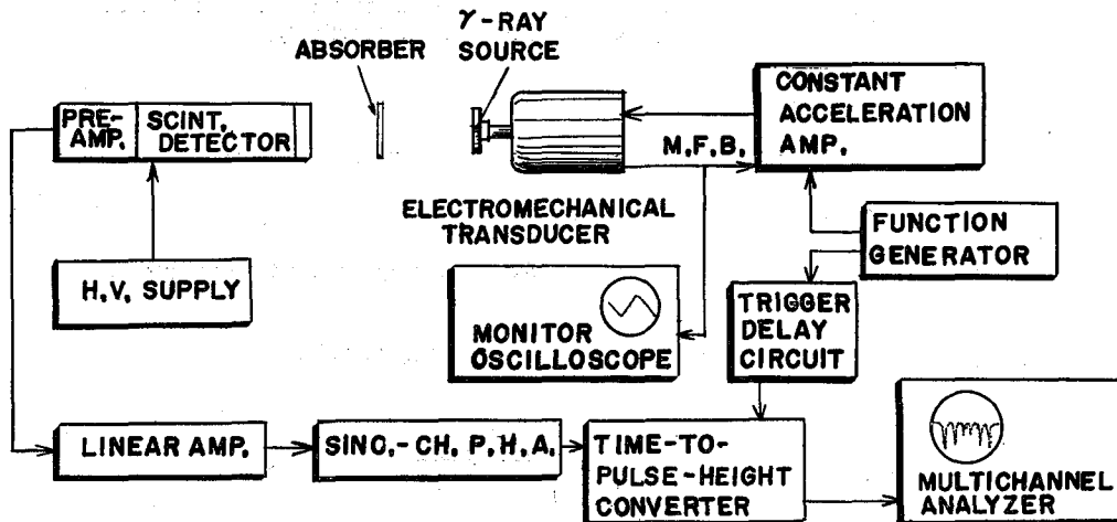
Fig. 1. Block diagram of the Mössbauer spectrometer.
