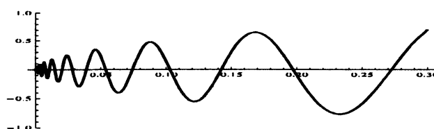
Figure 1: oscillations near x = 0
