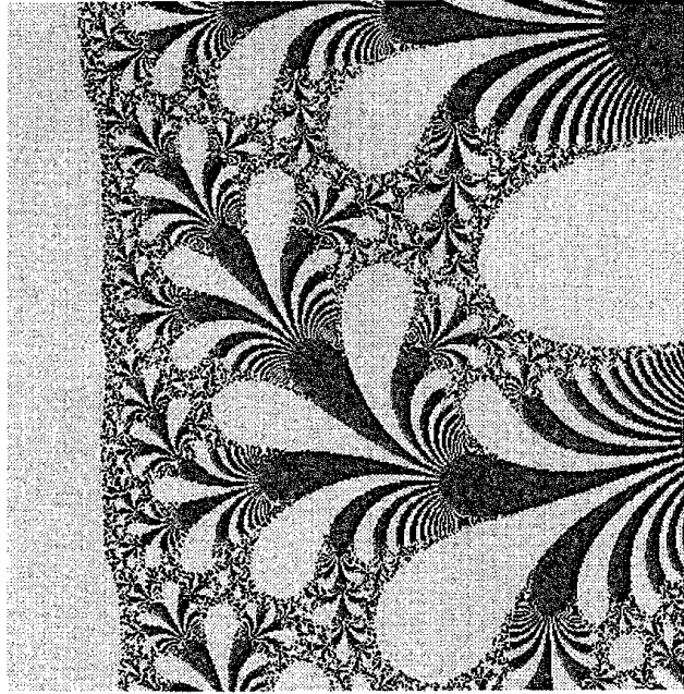
Figure 2: The Julia set of E_{a,b} , where a = -0.952639\cdots + i0.114414\cdots and b = -3.08884\cdots + i7.46149\cdots which satisfy the equations in Example 2. It has a superattracting fixed point 2.08884\cdots - i7.46149\cdots . The range shown is -7 < \Re z < 3 and -8 < \Im z < 2 .
