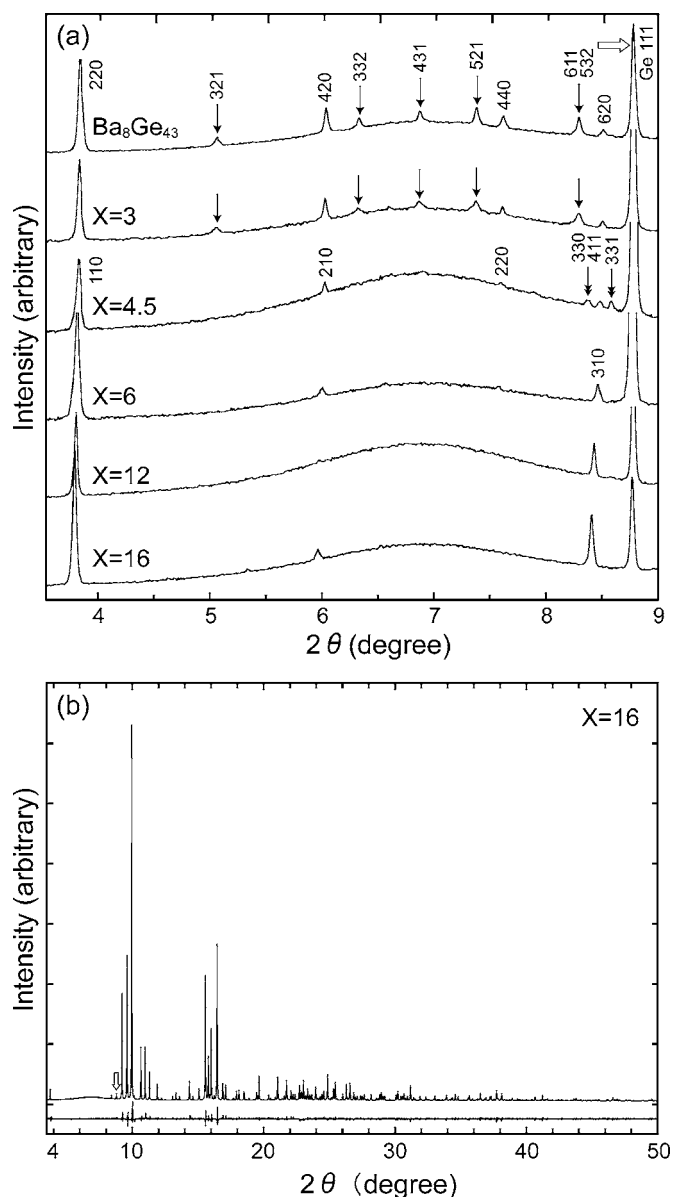
FIG. 2. (a) X-ray powder diffraction patterns in the 2\theta range from 3.5^\circ to 9^\circ for the oil-quenched specimen with X=3 and furnace-cooled specimens with X=4.5 , 6, 12, and 16. The pattern for the binary type-I clathrate compound Ba 8 Ge 43 is also shown for comparison. The solid arrows indicate superlattice reflections, while open and double arrows indicate reflections from Ge and type-III clathrate phases, respectively. (b) X-ray powder diffraction pattern in the 2\theta range from 3.5^\circ to 50^\circ for the specimen with X=16 .
