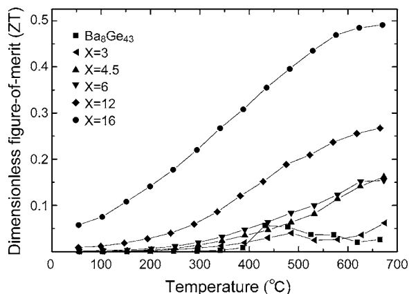
FIG. 6. Dimensionless figure of merit (ZT) for the specimens with X=0-16 plotted as a function of temperature.
