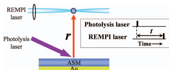
FIG. 1. Schematic illustration of the experiment. Photofragments from the 157 nm photodissociation of ASM are detected by the REMPI technique. The timing plot for measurements of a TOF spectrum is shown in the inset where the delay time t between photolysis and probe laser pulses corresponds to the TOF. r is the vertical distance between the disk substrate and the REMPI detection point. The VUV photoirradiated area is a disk with a radius of 6 mm.
