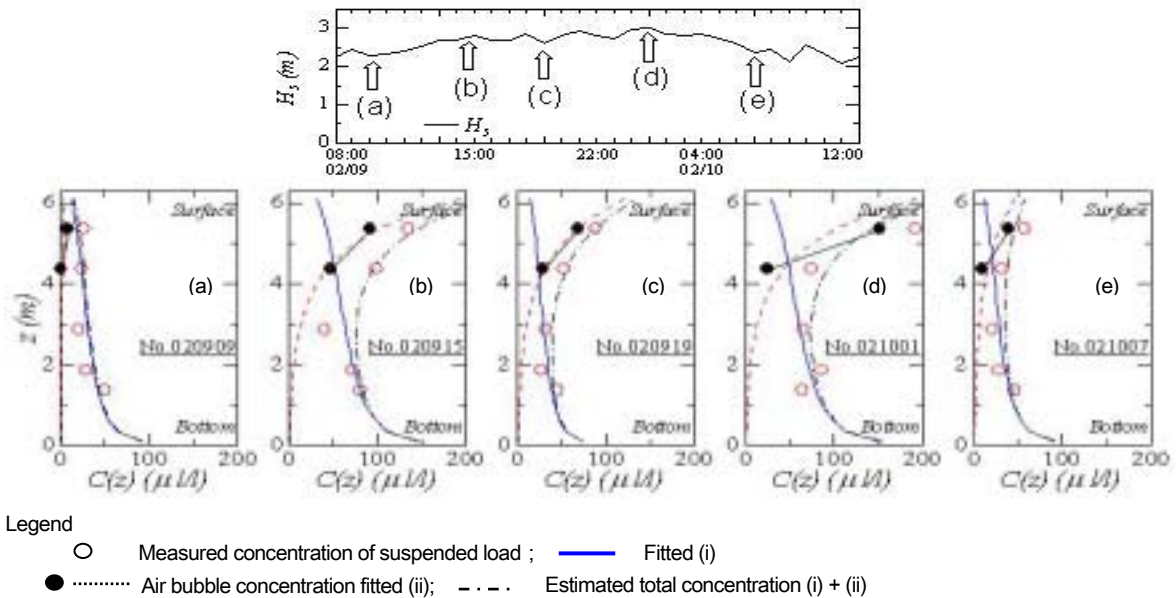
Fig.11. Measured profile of concentrations of suspended load and air bubble (Kato et al., 2002b)
