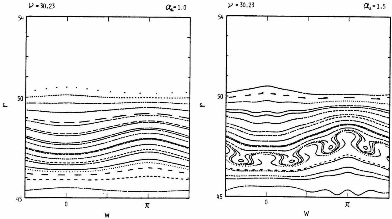
Fig.5.12 Numerically calculated phase points for \nu = 30.23 .
