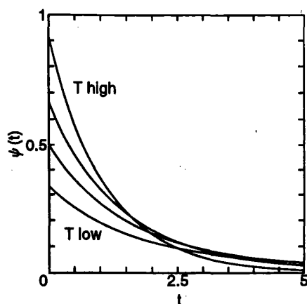
Fig. 1. A schematic plot of the waiting time distribution (WTD) for various temperatures. While the WTD decays rapidly for higher temperatures, it acquires a long tail for lower temperatures.
