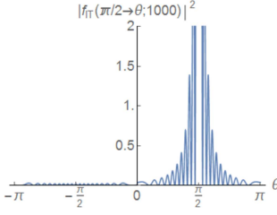
Figure 5: DSCS by the Ito–Tamura formula, \tau = \pi/2 .
