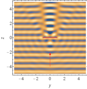
Figure 9: The density plot of \text{Re } \varphi_{-,1} .
