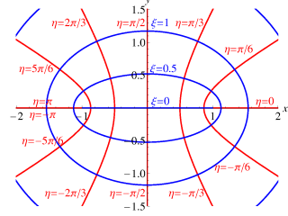
Figure 2: Elliptic coordinate.
