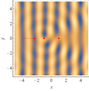
Figure 3: Plot of \text{Re } \varphi_- , for k = 4, \tau = 0 .
