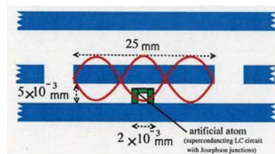
Figure 2: How to make the interaction between the artificial atom and the 1-mode photon of the microwave resonator.
