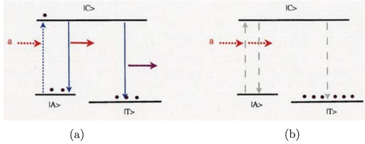
Figure 4: (a) Irradiation of the laser a to the 3-level system. (b) EIT and the dark state.
