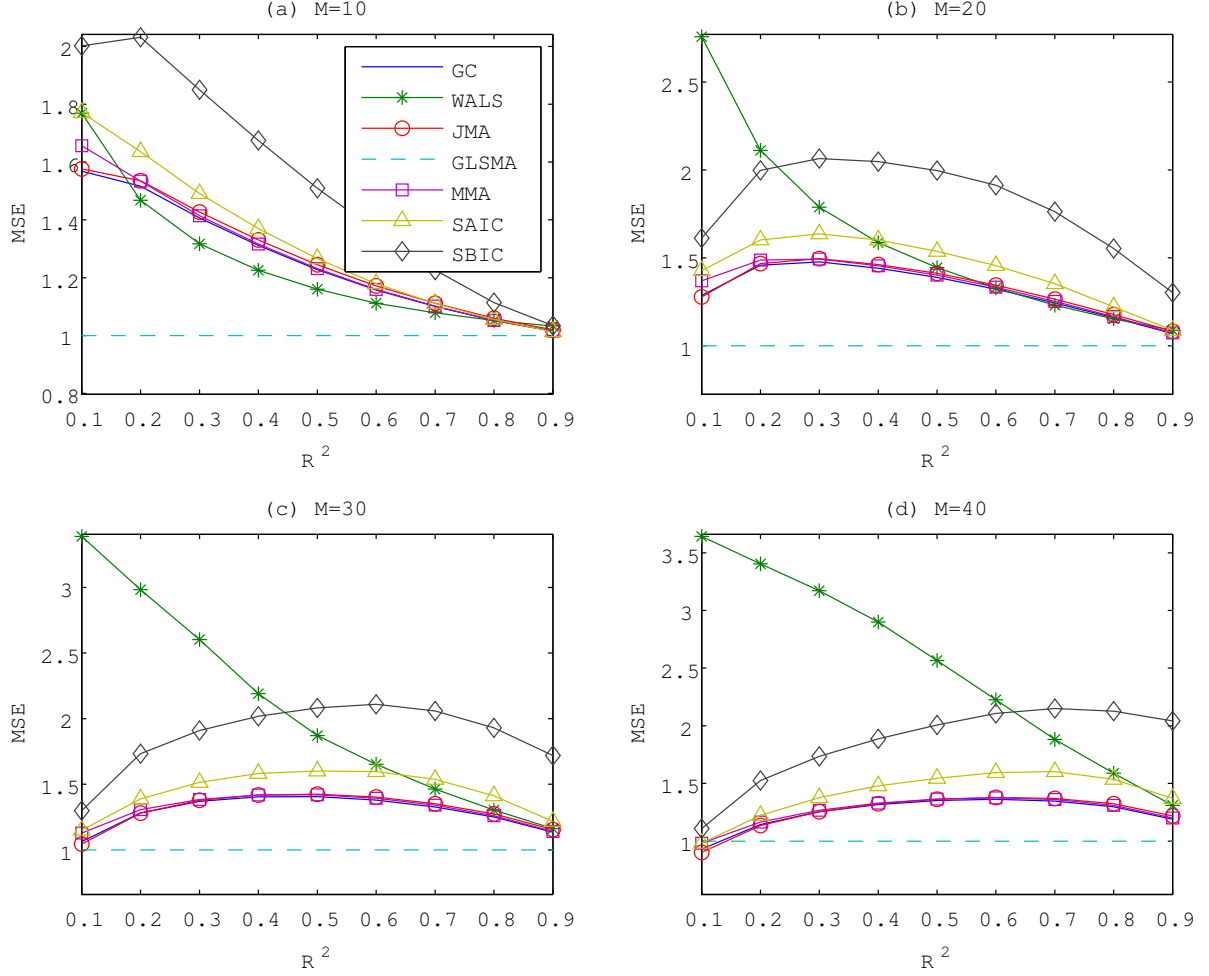
Figure 5: Performance of the FGLSMA estimator with nonparametric variance estimates based on C_{I_n}^F(W) and alternative estimators in the heteroskedastic design with n = 150 .
