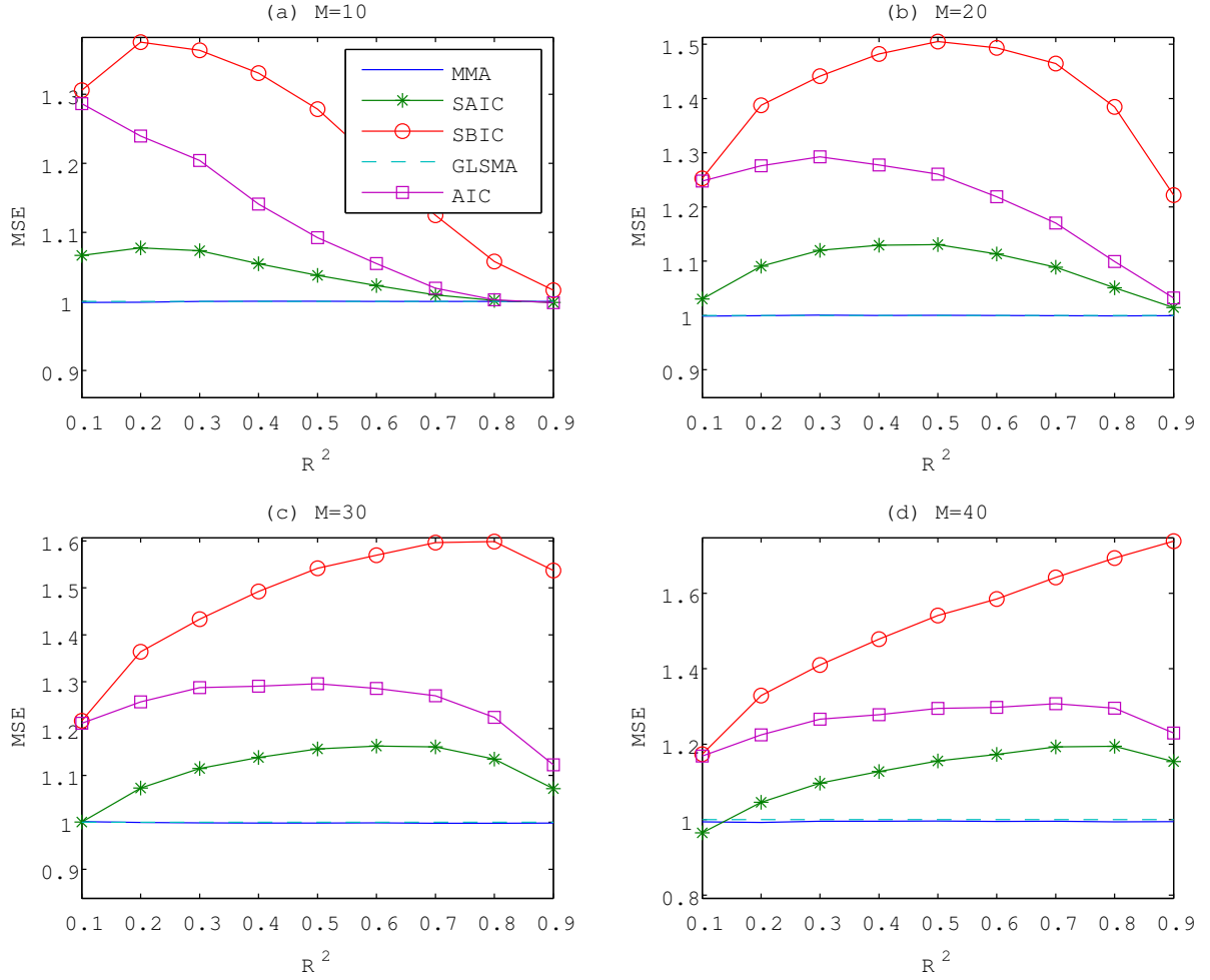
Figure 3: Performance of the FGLSMA estimator based on C_{I_n}^F(W) and alternative estimators in the homoskedastic design with n = 150 .
