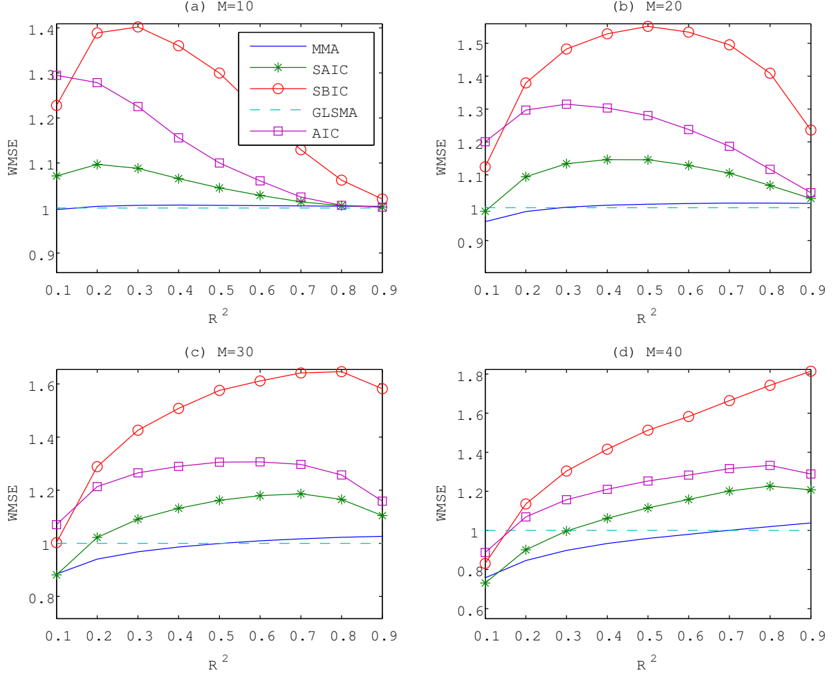
Figure 4: Performance of the FGLSMA estimator based on C_{\Omega}^F(W) and alternative estimators in the homoskedastic design with n = 150 .
