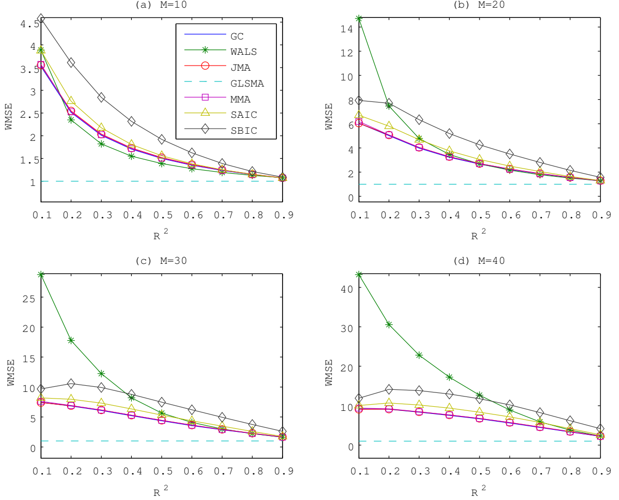
Figure 2: Performance of the FGLSMA estimator based on C_\Omega^F(W) and alternative estimators in the heteroskedastic design with n = 150 .
