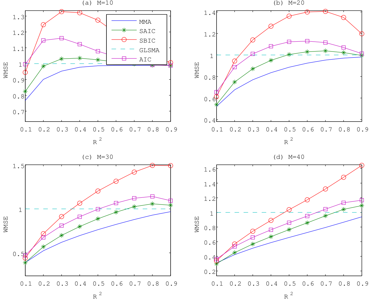
Figure 8: Performance of the FGLSMA estimator with nonparametric variance estimates based on C_\Omega^F(W) and alternative estimators in the homoskedastic design with n = 150 .
