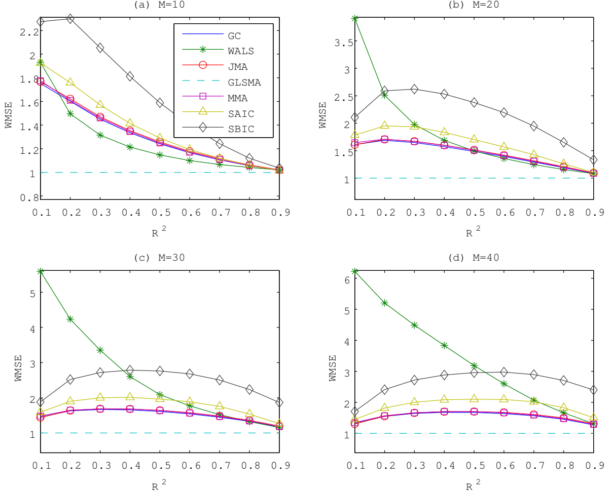
Figure 6: Performance of the FGLSMA estimator with nonparametric variance estimates based on C_{\Omega}^F(W) and alternative estimators in the heteroskedastic design with n = 150 .
