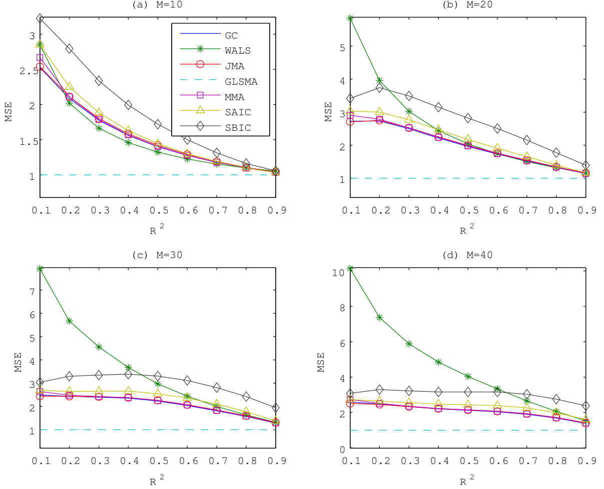
Figure 1: Performance of the FGLSMA estimator based on C_{I_n}^F(W) and alternative estimators in the heteroskedastic design with n = 150 .
