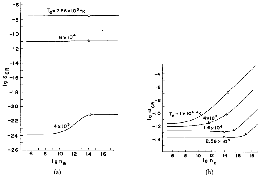
Fig. 9. (a) Collisional-radiative coefficient S_{CR} in the case B. Critical density: \odot ; Eqs. (45) and (44). (b) Coefficient \alpha_{CR} in the case B. Critical densities: \odot ; n_e^{\alpha\infty'} = A(3, 2)/F(3, 2) , \blacktriangle ; n_e^{\alpha\infty'} = \beta(1)/Z(1) \sum_{q \geq 2} C(1, q) .
