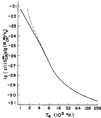
Fig. 7. Limiting value Z(1)S_{CR}^{\infty} \equiv \alpha_{CR}^{\infty}/n_e ( \text{cm}^6 \text{ sec}^{-1} ) vs. T_e ( 10^3 \text{ } ^\circ\text{K} ). —; the bottom row in Table 2(b), ---; Eq. (38') or (39'). See also Figs. 2(a) and (b).
