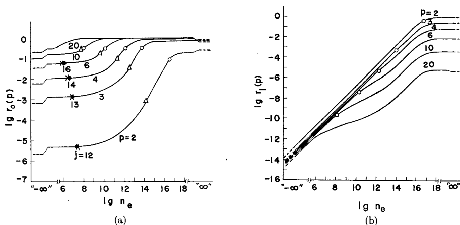
Fig. 1. (a) Population coefficient r_0(p) vs. n_e (cm -3 ) for T_e=4 \times 10^3 °K. Critical electron densities: ●; Eqs. (12), (13) and (17), where j is indicated, ×; Eq. (18). △; Eq. (14), ○; Eq. (17). Limiting values: for \lg n_e \rightarrow -\infty , —; the top row in Table 1, ---; Eq. (22). For \lg n_e \rightarrow \infty , —; the bottom row in Table 1, ---; Eq. (25). (b) Population coefficient r_1(p) vs. n_e (cm -3 ) for T_e=4 \times 10^3 °K. Critical densities; ○; Eqs. (20) and (17). Limiting values: for \lg n_e \rightarrow -\infty , —; the top row in Table 1, ---; Eq. (23). For \lg n_e \rightarrow \infty , —; the bottom row in Table 1, ---; Eq. (28) with (29).
