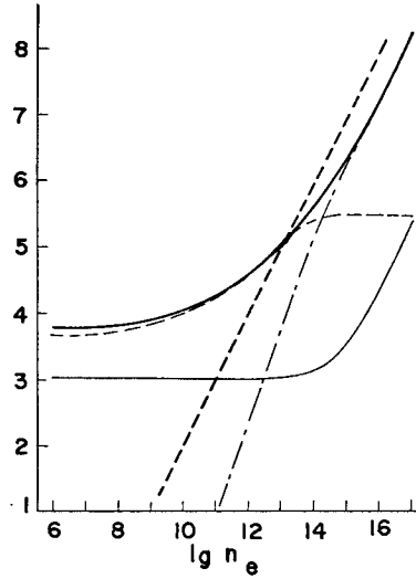
Fig. 10. Contributions from various terms in Eq. (10) for r_0(2) in the case B. T_e = 4 \times 10^3 °K. Ordinate shows following values in logarithmic scale. ---; denominator, \{F(2, 1) + \sum_{q \geq 3} C(2, q) + S(2)\} n_e . —; numerator, —; \{\alpha(2)n_e + \beta(2)\} / Z(2) , - - - -; \sum_{q \geq 3} Z(q) r_0(q) F(q, 2) n_e / Z(2) , - - -; \sum_{q \geq 3} Z(q) r_0(q) A(q, 2) / Z(2) .
