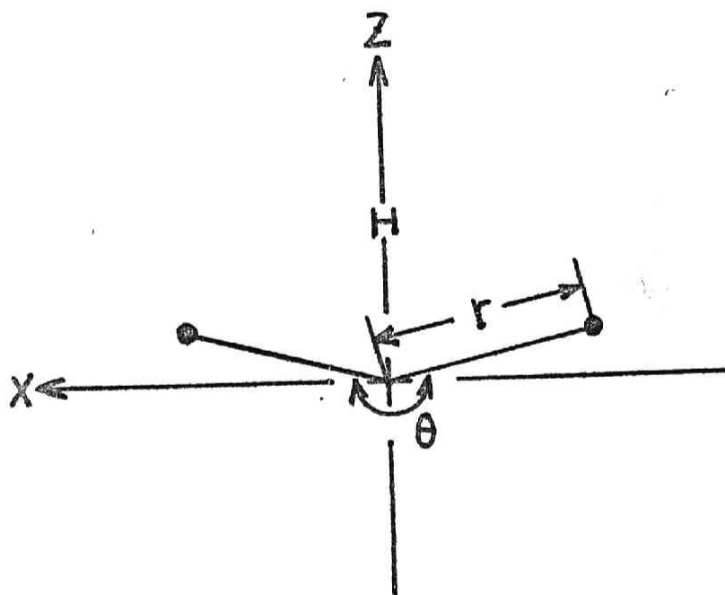
FIG. 1. The coordinates of the centers of two floating functions in \text{H}_2\text{O} molecule. Each center is indicated by a solid circle and is on the x-z plane. The H in the figure indicates the projected position of H nucleus to the x-z plane. The r indicates a distance between O nucleus (at origin) and the center of a floating function. The \theta is the angle between two centers as is shown in the figure.
