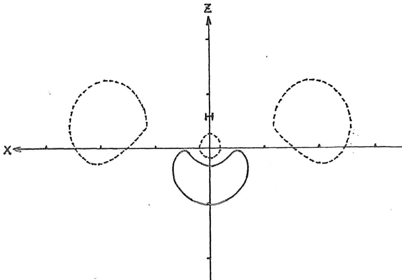
FIG. 6. The first non-bonding excited orbital (NBEO) listed in Table XIII for \text{H}_2\text{O} molecule. For coordinates and H in the figure, see the caption of Fig. 1.
