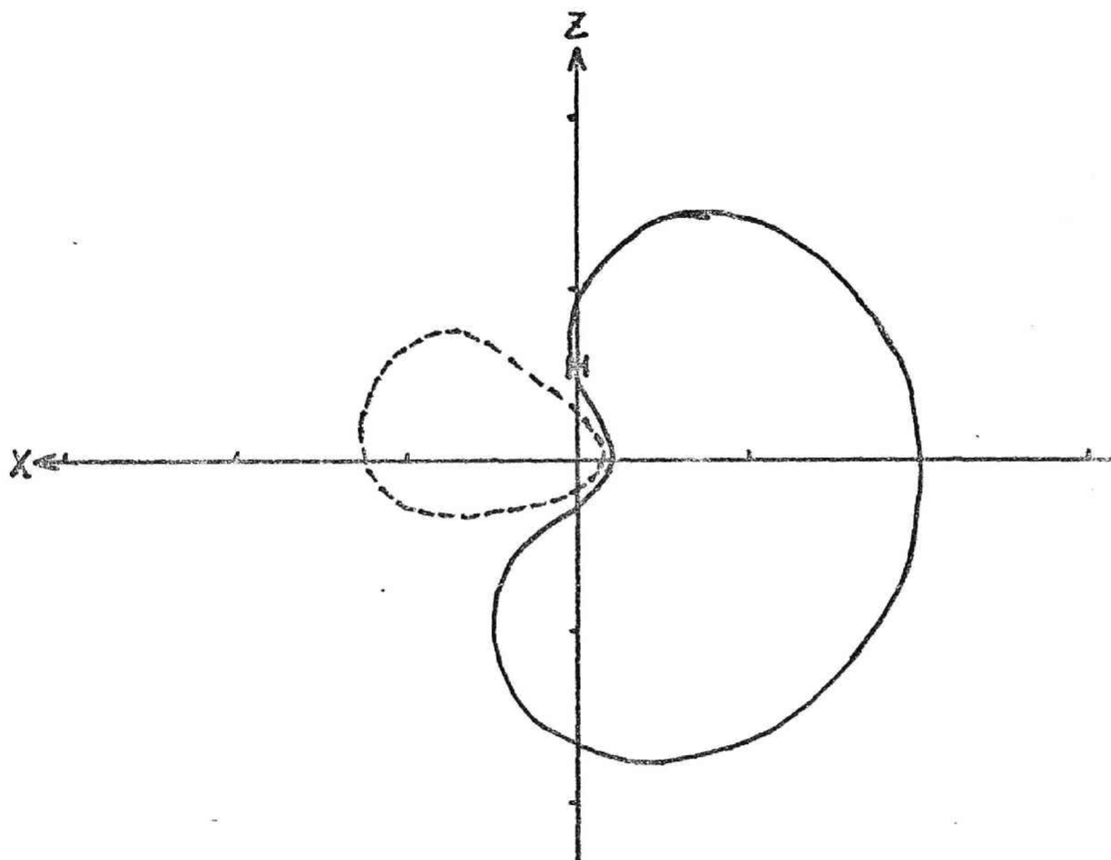
FIG. 9. One of the non-bonding orbitals listed in Table XIV for \text{H}_2\text{O} molecule. For coordinates and H in the figure, see the caption of Fig. 1.
