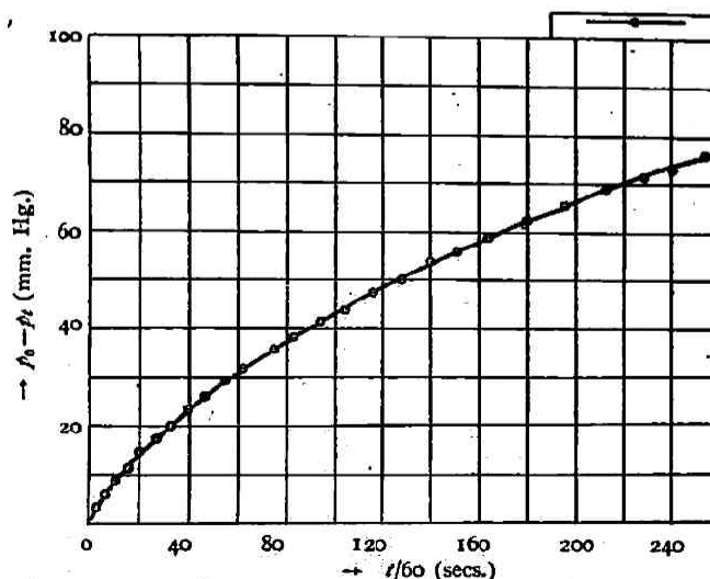
Fig. 8. Decomposition of carbon monoxide at 350°C. in the presence of catalyst IV saturated with carbon dioxide.
