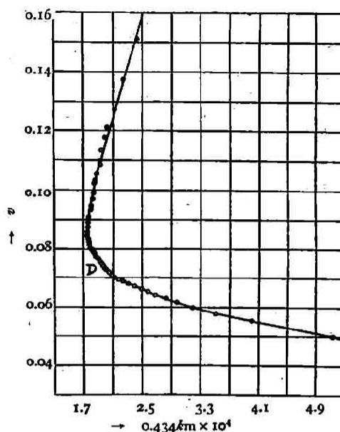
Fig. 7. Chemisorption of carbon dioxide by catalyst III b at 330°C.
