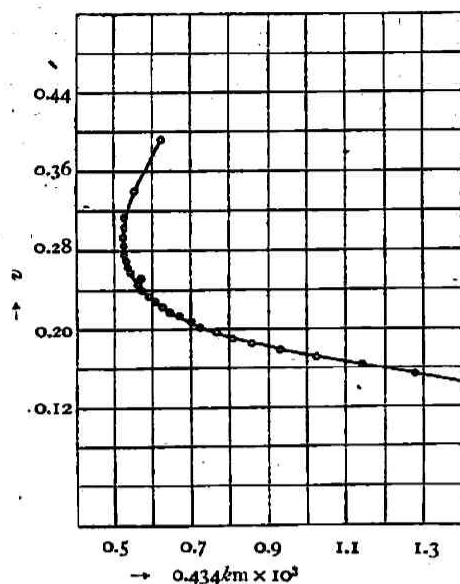
Fig. 6. Chemisorption of carbon dioxide by catalyst III a at 350°C.
