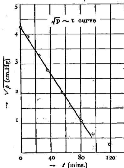
Fig. 5. \sqrt{p} \sim t curve for the chemisorption of carbon dioxide by catalyst V at 360^\circ\text{C} .
