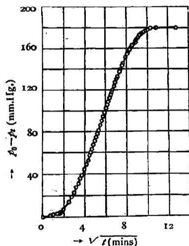
Fig. 4. (p_0 - p) \sim \sqrt{t} curve for the chemisorption of carbon dioxide by catalyst V at 360^\circ\text{C} .
