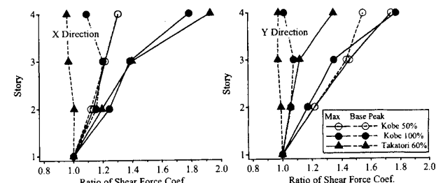
Figure 6 Distribution of story shear force coefficient
