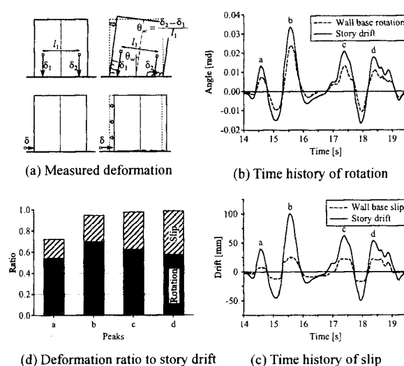
Figure 2 Deformation of wall base (JMA-Kobe 100%)
