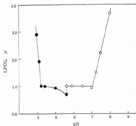
Fig. 2 Effect of pH on LPCG of pressure gelation
