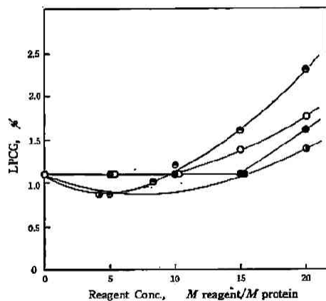
Fig. 7 Effects of alkylating and mercuptide reagents on LPCG of thermal gelation by heating for 15 min. at 97-99^\circ\text{C} , in the presence of iodoacetate (●), iodoacetamide (●), mercuric chloride (○), and p -chloromercuribenzoate (○).
