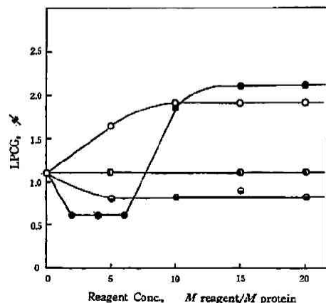
Fig. 8 Effects of oxidizing and reducing reagents on LPCG of thermal gelation. The sample solution were heated for 15 min. at 97-99^\circ\text{C} , in presence of potassium ferricyanide (●), potassium iodide (●), and iodine in potassium iodide (○), and cysteine (○). The pH was adjusted to 7.0 with phosyphate buffer (0.1M).
