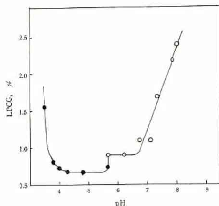
Fig. 1 Effect of pH on LPCG of thermal gelation
