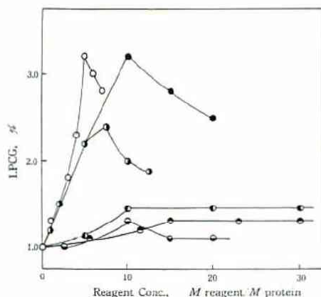
Fig. 5 Effects of sulfhydryl reagents on the LPCG of pressure gelation
