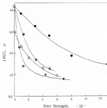
Fig. 4 Effects of salts on LPCG's of thermal gelation and of pressure gelation
