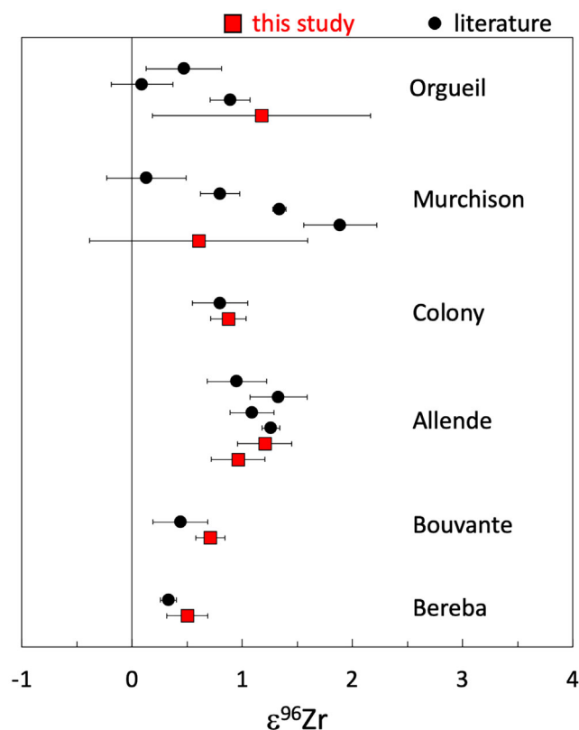
FIGURE 2. The \epsilon^{96}\text{Zr} data for several meteorites. Data are from Table 1 using \epsilon^{96}\text{Zr}_{(99 \text{ corr.})} and from Akram et al. (2013, 2015); Elfers et al. (2020); Render and Brennecke (2021); Render et al. (2022). The data of Akram et al. (2013, 2015), originally analyzed against an Alfa Aesar Zr standard, were recalculated relative to NIST SRM 3169 Zr using the values from Akram and Schönbachler (2016). Uncertainties are given as 2SE for data from this study and as 95% CI for data from Render and Brennecke (2021) and Render et al. (2022), except if n < 5 , where the 2SD of Colony is used ( \pm 1 ) for data from this study and published 2SD for literature data. (Color figure can be viewed at wileyonlinelibrary.com )
