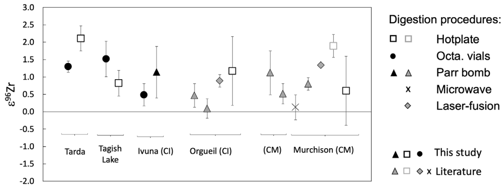
FIGURE 4. Comparisons of Zr isotope data of carbonaceous chondrites analyzed using different digestion methods during sample preparation. Uncertainties and data sources are the same as in Figure 2. Octa: octagonal-body Savillex ® vials.
