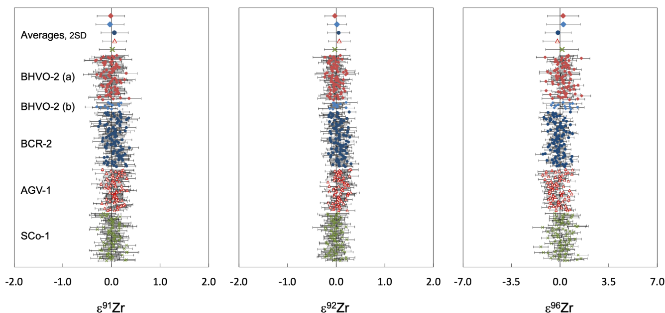
FIGURE 1. The Zr isotope data for five terrestrial rock reference materials. BHVO-2 (a) and (b) denote two different digestions. Shown are single measurements and their internal error (2SE) as well as the average of each sample with the corresponding uncertainty given as the 2 sd calculated from the individual sample measurements (Table 1 and Table S2). For \epsilon^{91}\text{Zr} , values using ^{99}\text{Ru} for Ru interference correction are shown. (Color figure can be viewed at wileyonlinelibrary.com )
