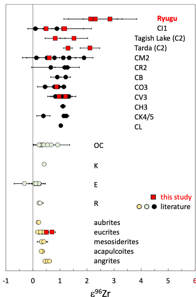
FIGURE 3. The \epsilon^{96}\text{Zr} data for bulk samples of Ryugu and various meteorite groups. The spread in the data is generally larger for meteorite groups that experienced higher degrees of aqueous alteration (types 1 and 2) compared with those with less alteration (e.g., CV3). Red symbols denote data from this study (Table 1 using \epsilon^{96}\text{Zr}_{(99 \text{ corr.})} ). Literature data are from the compilation published in Rüfenacht et al. (2023), summarizing results from Akram et al. (2013, 2015); Elfers et al. (2020); Render and Brennecke (2021); Render et al. (2022). Uncertainties are the same as in Figure 2. (Color figure can be viewed at wileyonlinelibrary.com )
