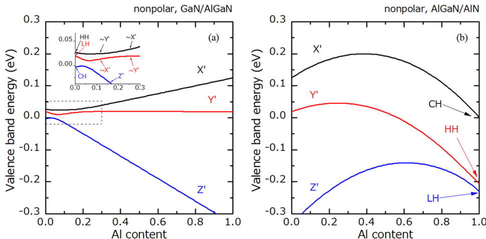
FIG. 4. (Color online) VB energy structure of (a) nonpolar GaN/Al y Ga 1-y N and (b) nonpolar Al x Ga 1-x N/AlN strained bulks. Origin of VB energy is set to the VB energy of an unstrained bulk crystal without crystal-field splitting and spin-orbit interaction. Inset in (a) magnifies the VB structure with an Al content from 0.0 to 0.3.
