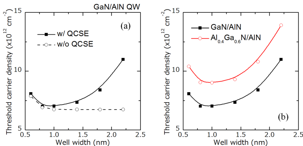
FIG. 3. (Color online) Well width dependence of the threshold carrier density of c -plane \text{GaN}/\text{AlN} QWs. (a) Threshold dependence on QCSE and (b) threshold dependence on Al content.
