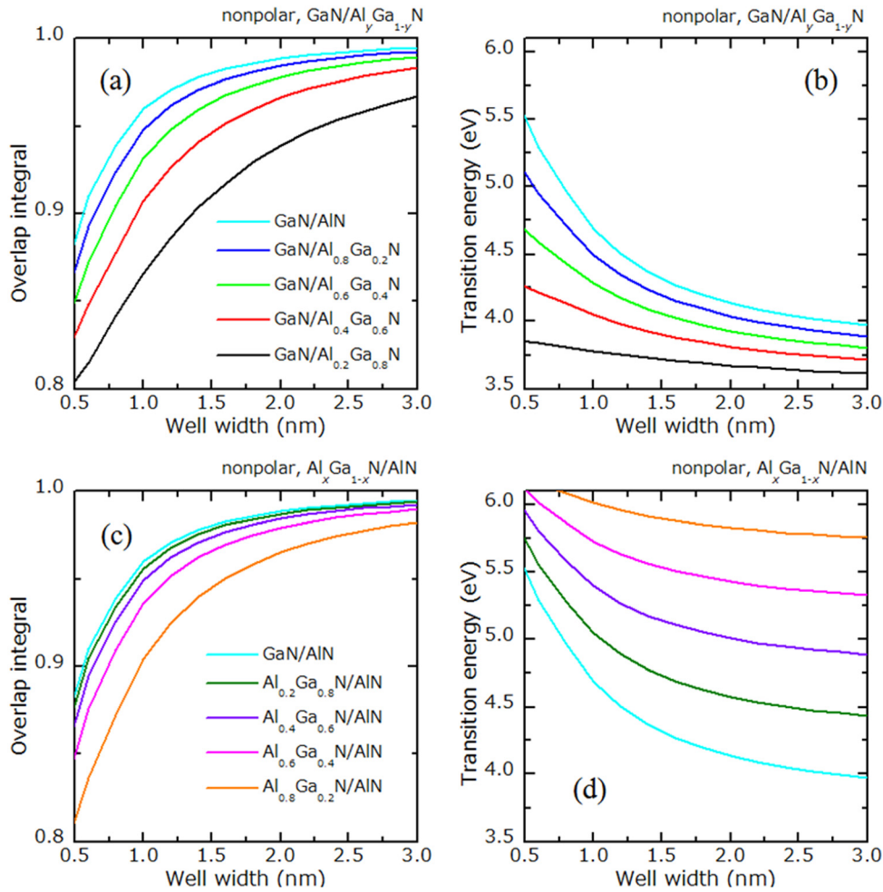
FIG. 5. (Color online) (a) Overlap integral of GaN/Al x Ga 1-x N QWs, (b) transition energy of GaN/Al x Ga 1-x N QWs, (c) overlap integral of Al x Ga 1-x N/AlN QWs, and (d) transition energy of Al x Ga 1-x N/AlN QWs. Crystal orientation is the nonpolar plane.
