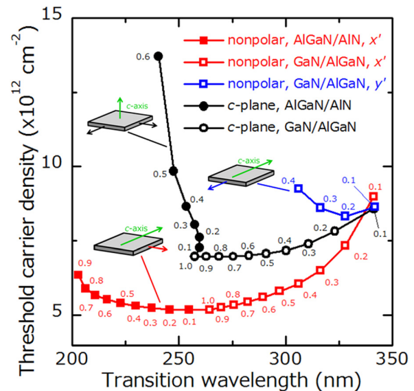
FIG. 8. (Color online) Threshold carrier density of 1-nm-thick \text{Al}_x\text{Ga}_{1-x}\text{N}/\text{Al}_y\text{Ga}_{1-y}\text{N} QWs. Black, red, and blue lines represent the threshold for c -plane QWs, nonpolar QWs with E \parallel c ( x' -polarization), and nonpolar QWs with E \perp c ( y' -polarization), respectively. Small numbers indicate Al content.
