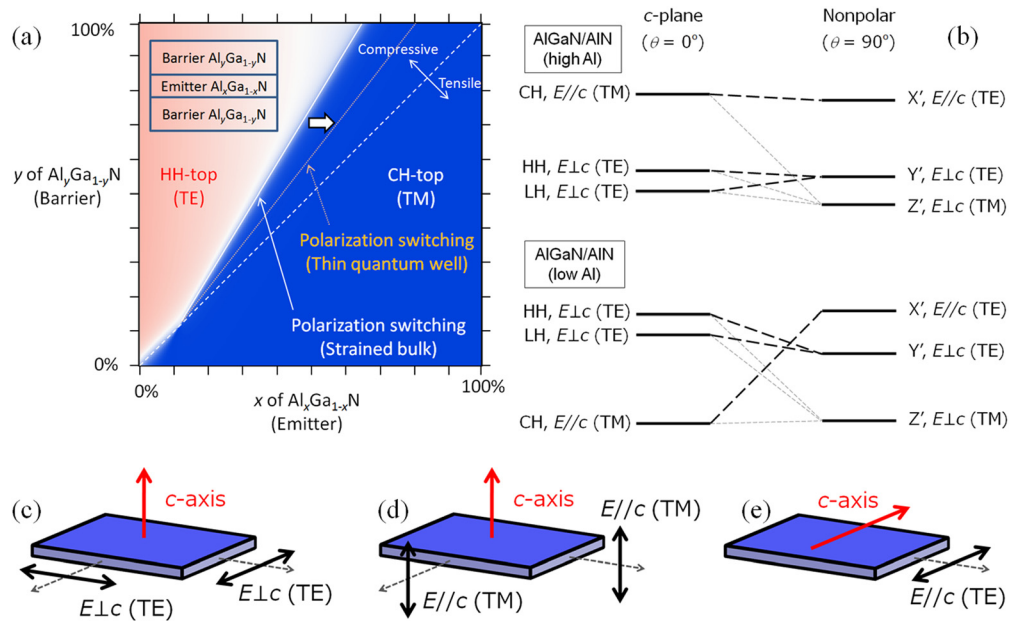
FIG. 1. (Color online) (a) Diagram of the top VB of a c -plane \text{Al}_x\text{Ga}_{1-x}\text{N} / \text{Al}_y\text{Ga}_{1-y}\text{N} heterostructure. (b) VB line-up of \text{AlGaIn/AlN} on the c -plane and nonpolar plane. Possible geometries of LD cavities for (c) c -plane \text{AlGaIn/AlN} with a low Al content, (d) c -plane \text{AlGaIn/AlN} with a high Al content, and (e) nonpolar \text{AlGaIn/AlN} ( x' polarization) where red solid, black solid, and black dashed arrows represent the c -axis, electric-field, and propagation direction of light, respectively.
